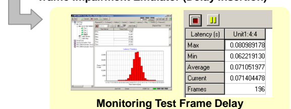
Fig. 3: Delay Insertion
