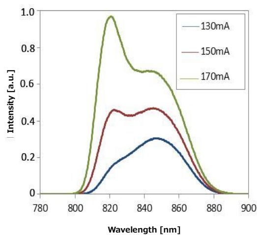
Emission Spectrum
