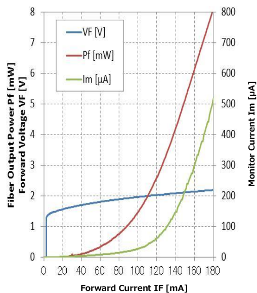
Output Power / Forward Voltage / Monitor Current
