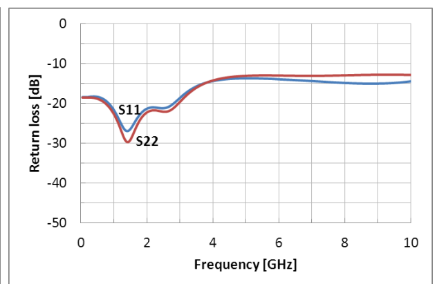
Reflection characteristics
