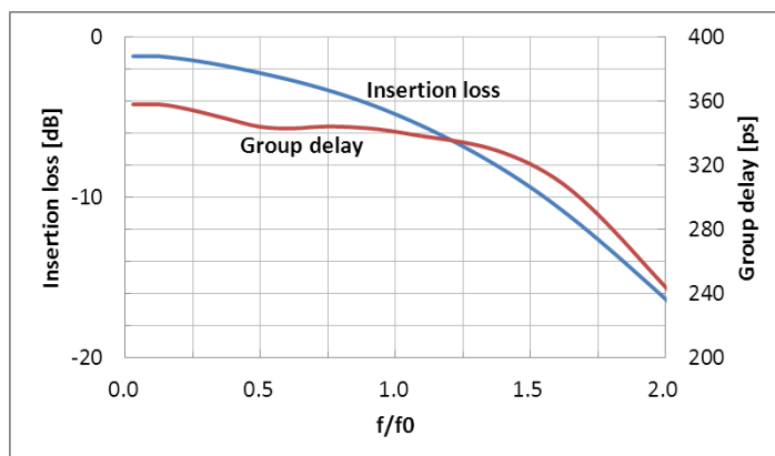
Transmission characteristic
