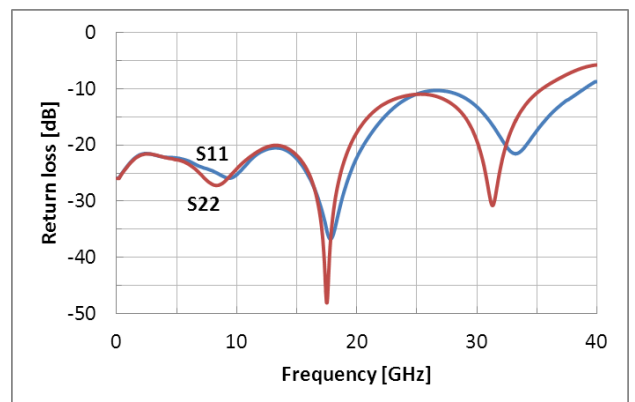
Reflection characteristics
