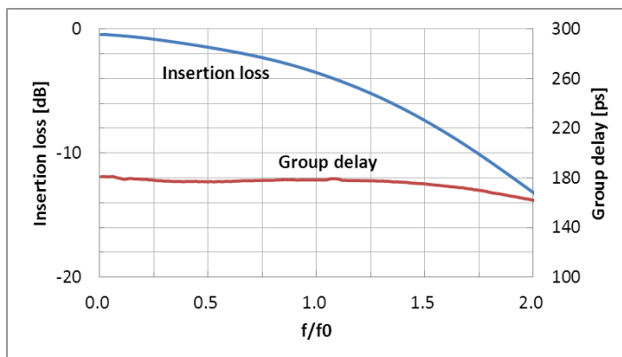
Transmission characteristic
