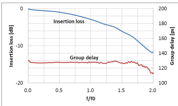
Transmission characteristic
