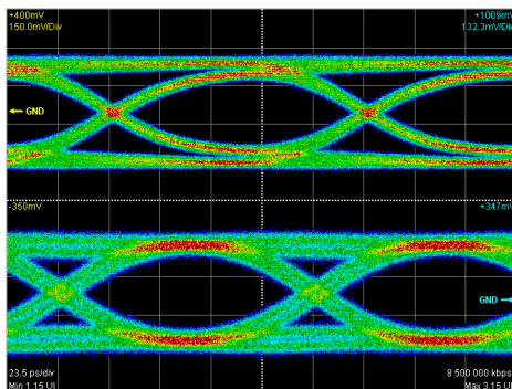
Actual waveforms (EYE) (Bit Rate: 8.5Gbit/s, Pattern: PRBS 31)
