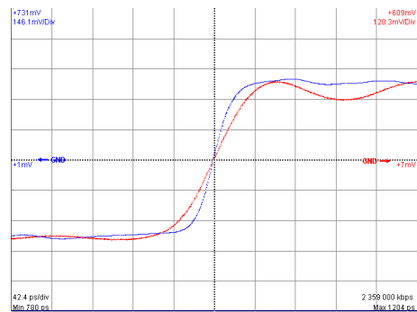
Actual waveforms (Pulse) (Bit Rate: 2.25Gbit/s, Pattern: 01 signals) Rise Time: 17.00 (SMA) 40.16 (probe)
