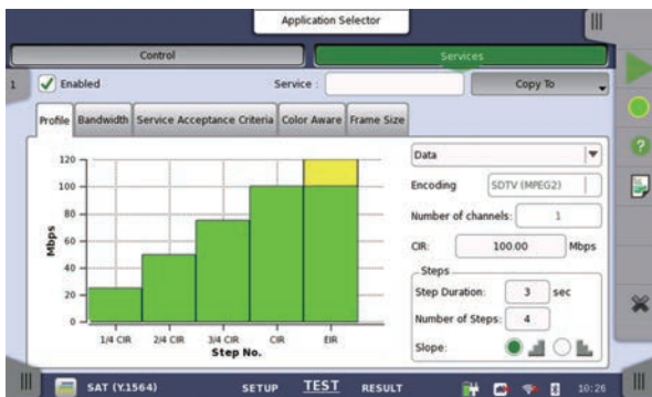
Simple and intuitive configuration of Y.1564 test
