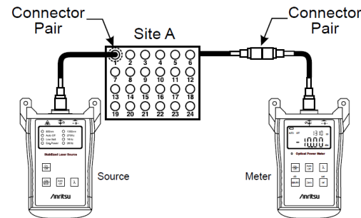
Figure 3 Patch Panel to Connector
