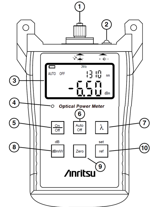
Figure 1 CMA5 Series Power Meter Operating Controls
