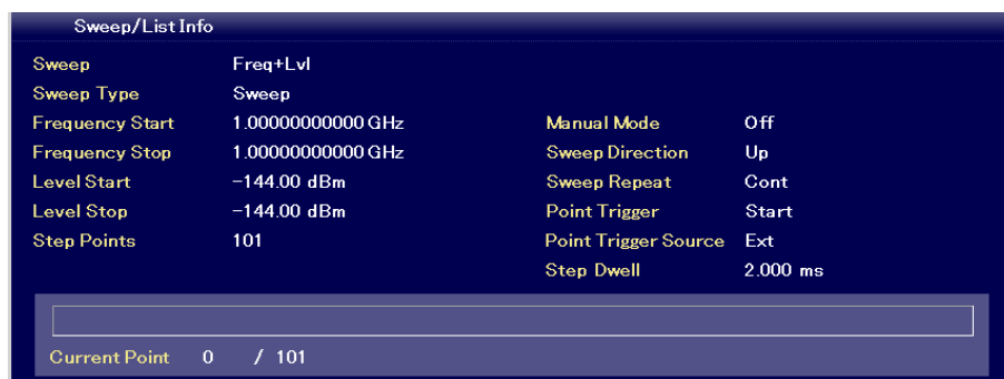
Figure 6.1.1-1 Sweep/List Info Dialog Box (Sweep Type : "Sweep")
