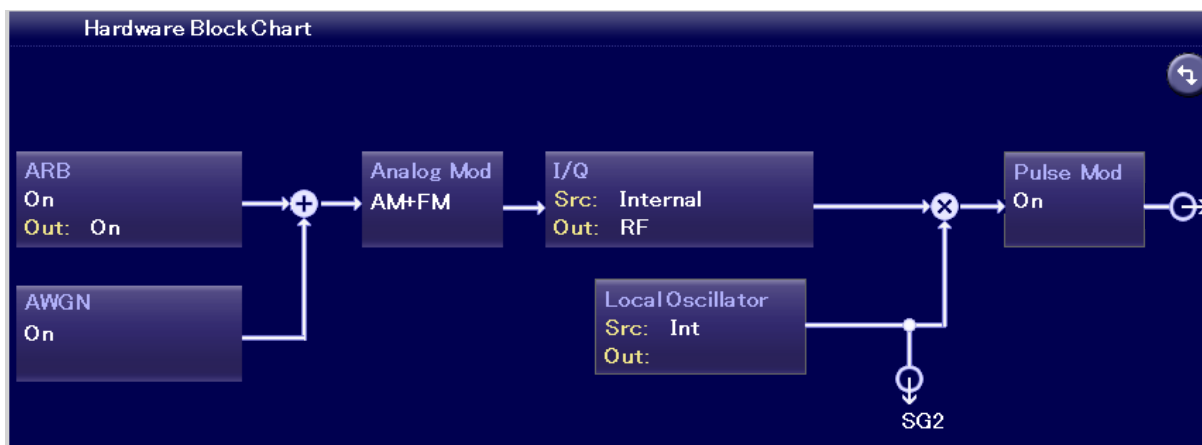
Figure 7.1-1 Outline of MG3710A/MG3710E/MG3740A modulation circuit
