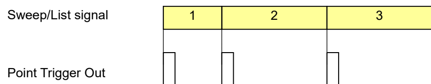
Figure 7.4.2-2 Point Trigger Out
