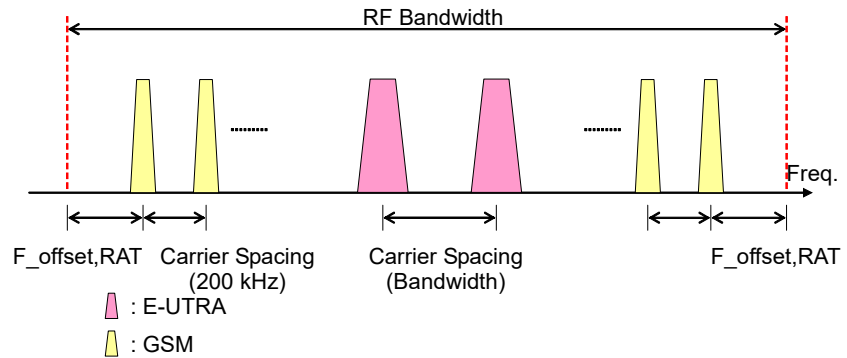
Figure 3.2.6-12 Carrier Allocation Of TC4b
