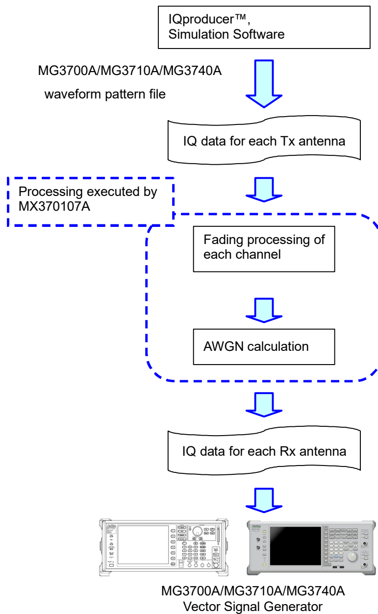
Fig. 1.1-1 Fading processing flow
