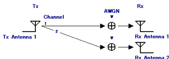
Figure 3.1.2.2-2 1 \times 2 SIMO configuration
