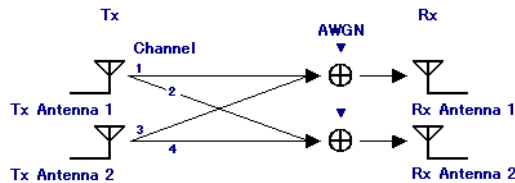
Figure 3.1.2.2-6 2 × 2 MIMO configuration
