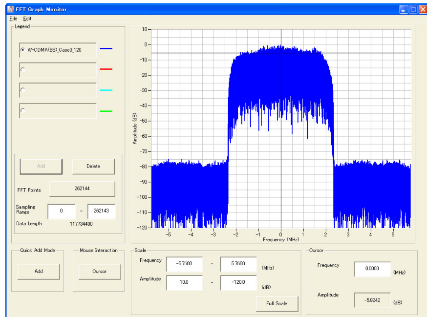
Figure 3.3.1-9 Spectrum (W-CDMA Case3 120km/h)
