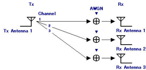
Figure 3.1.2.2-3 1 × 3 SIMO configuration
