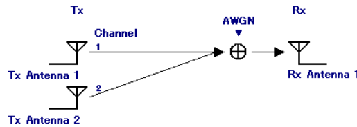
Figure 3.1.2.2-5 2 × 1 MISO configuration
