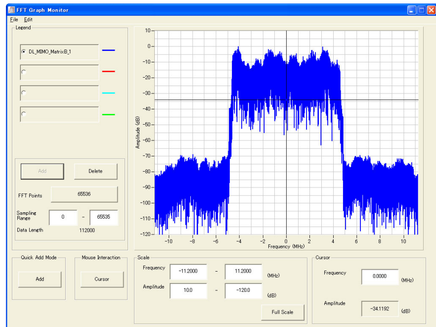
Figure 3.3.5-13 Spectrum (Rx Antenna 1)
