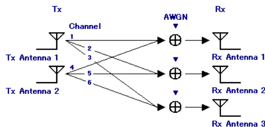
Figure 3.1.2.2-7 2 × 3 MIMO configuration
