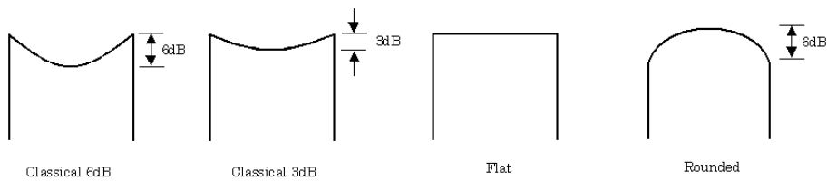
Figure 3.1.3-3 Doppler spectrum shapes
