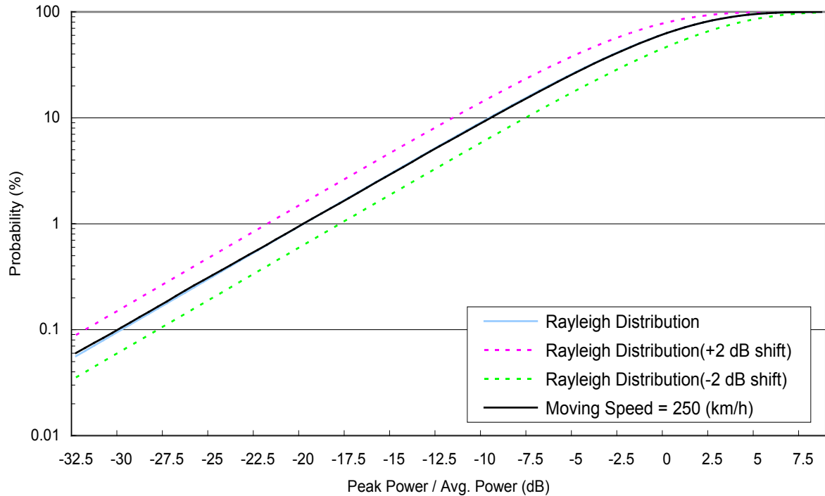
Figure D.2-7 Accumulated probability distribution (Moving Speed = 250 km/h)
