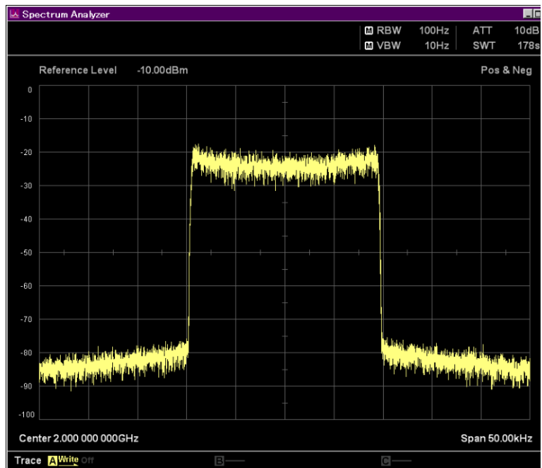
Figure D.1-1 Rayleigh with Classical 3 dB
