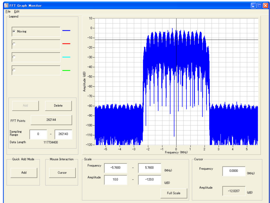
Figure 3.3.2-9 Spectrum (Moving Propagation)
