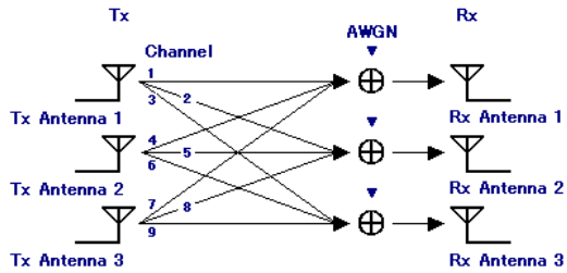
Figure 3.1.2.2-11 3 \times 3 MIMO configuration
