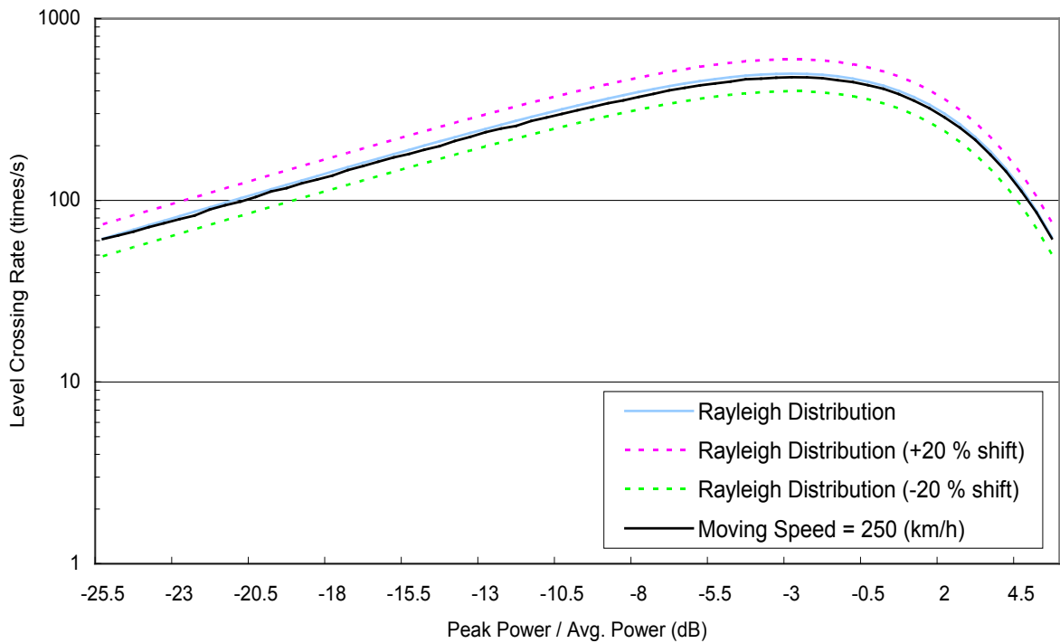
Figure D.2-8 Level crossing rate (Moving Speed = 250 km/h)
