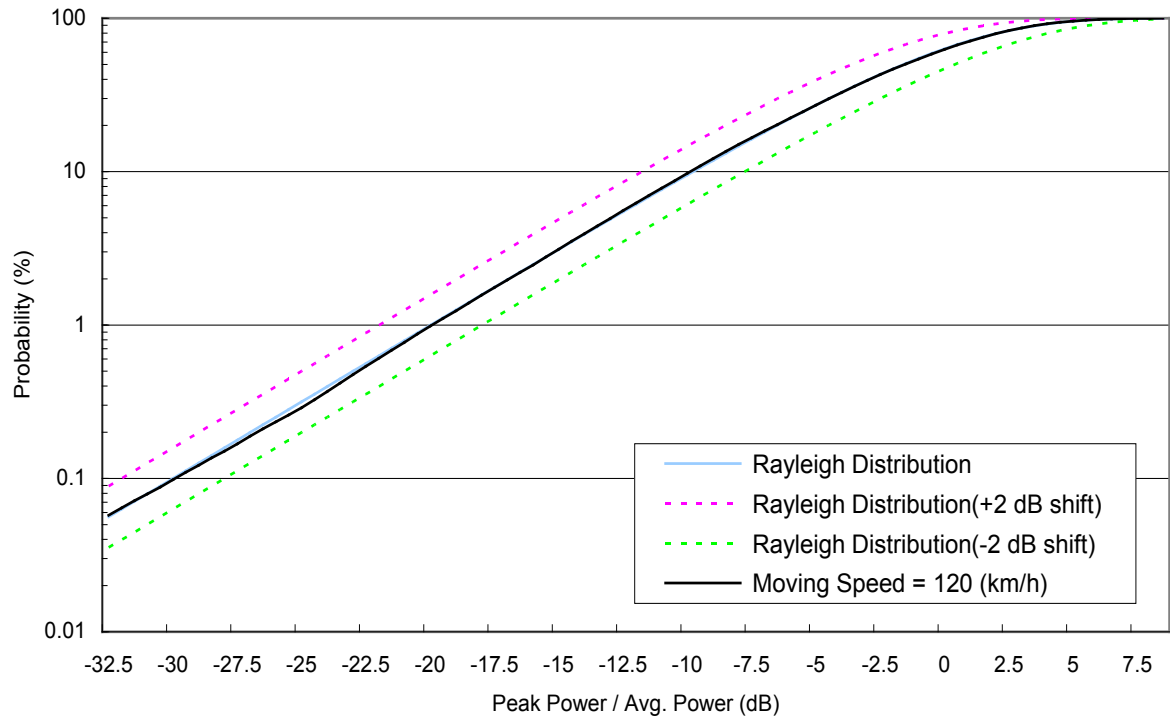
Figure D.2-5 Accumulated probability distribution (Moving Speed = 120 km/h)
