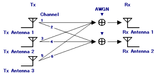
Figure 3.1.2.2-10 3 \times 2 MIMO configuration
