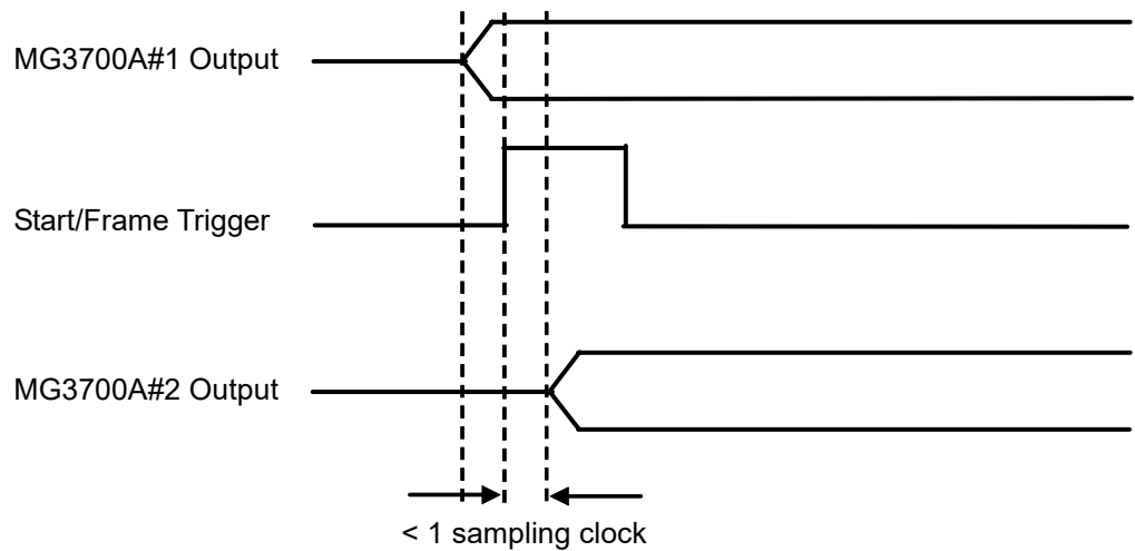
Figure C.1-5 Synchronization relationship of baseband signals when using Primary/Secondary
