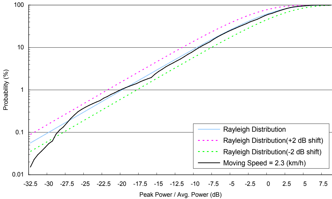
Figure D.2-1 Accumulated probability distribution (Moving Speed = 2.3 km/h)
