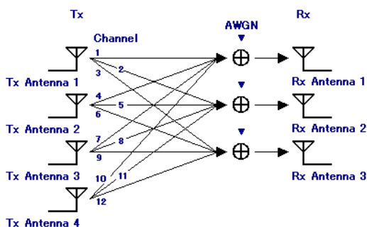
Figure 3.1.2.2-15 4 \times 3 MIMO configuration
