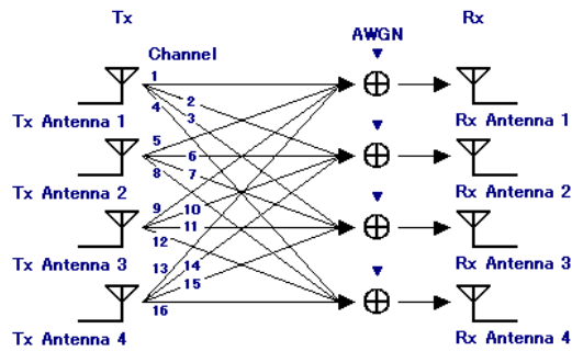
Figure 3.1.2.2-16 4 \times 4 MIMO configuration
