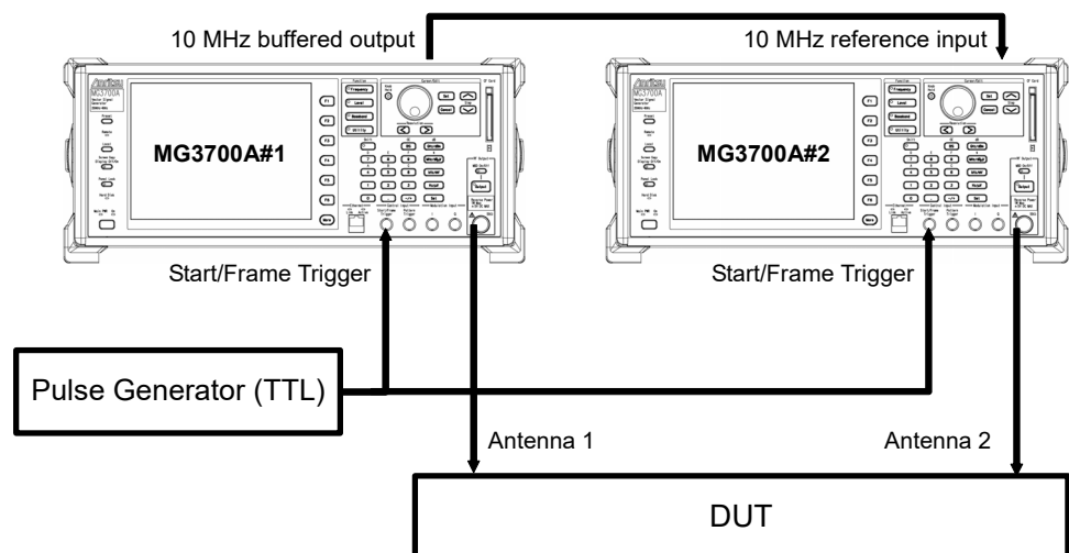
Figure C.1-1 Multiple MG3700A connection (external Start/Frame Trigger)
