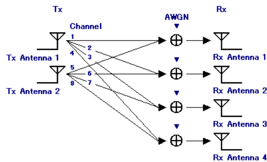
Figure 3.1.2.2-8 2 \times 4 MIMO configuration
