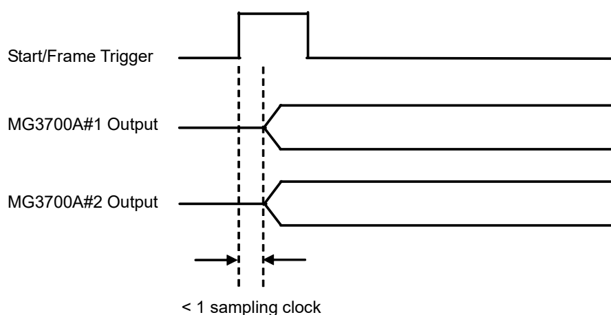
Figure C.1-2 Synchronization-baseband signals when using external Start/Frame Trigger
