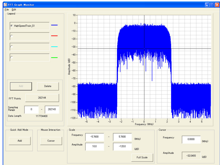
Figure 3.3.4-9 Spectrum (High Speed Train (Scenario1))
