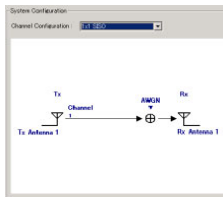
Figure 3.3.4-1 System Configuration (1 × 1 SISO)
