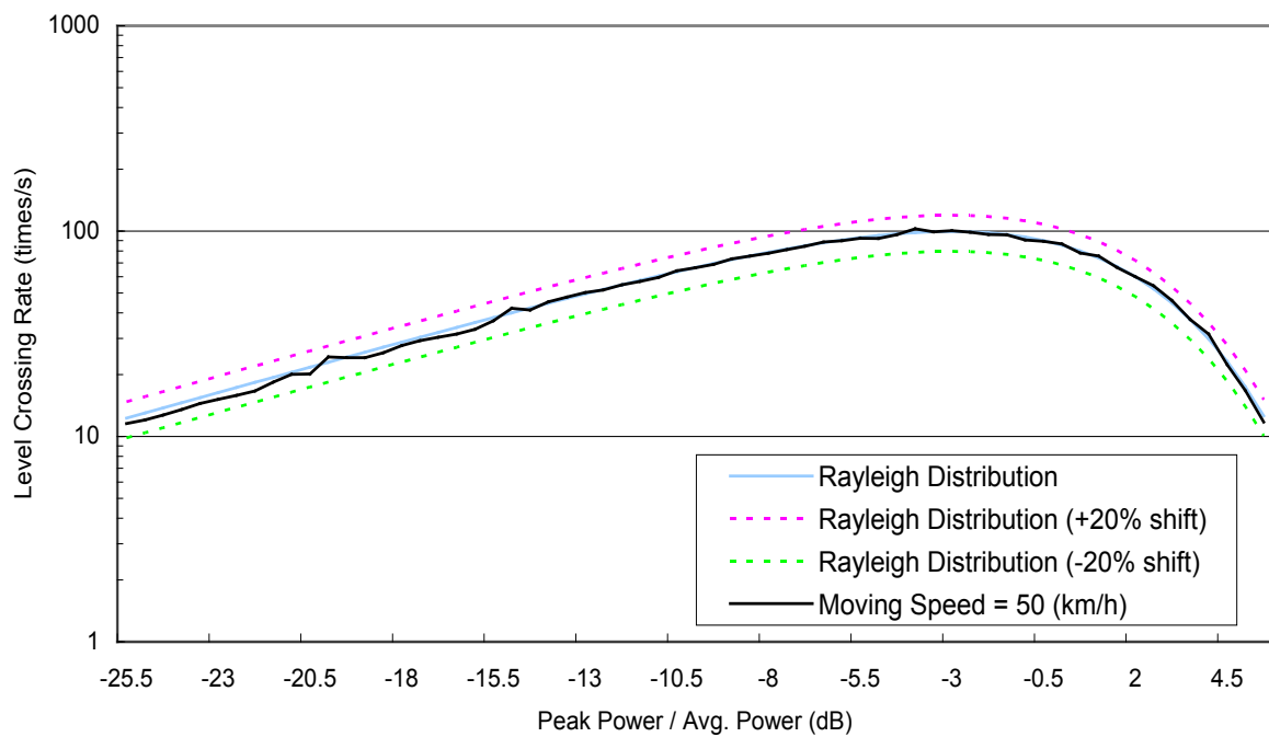
Figure D.2-4 Level crossing rate (Moving Speed = 50 km/h)
