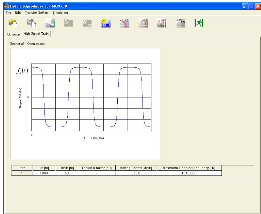
Figure 3.1.6-1 High Speed Train tab window (Scenario1)
