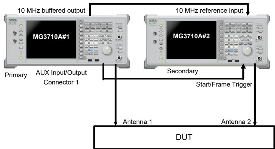
Figure C.2-4 Multiple MG3710A connection (Primary/Secondary)
