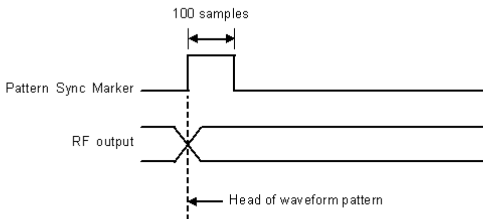
Figure 3.5-1 Pattern Sync Marker signal and RF output
