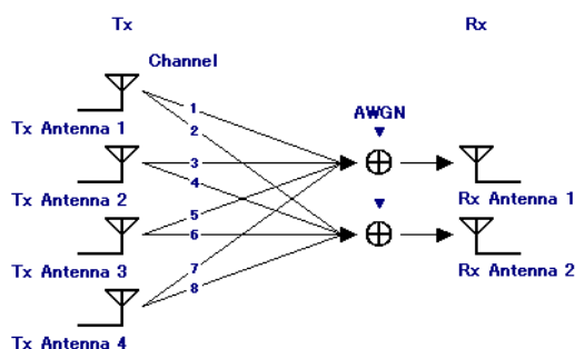
Figure 3.1.2.2-14 4 \times 2 MIMO configuration
