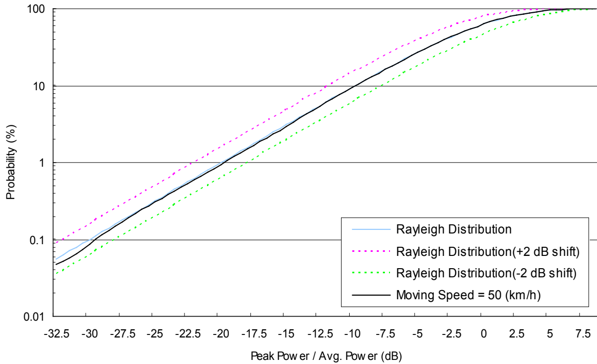
Figure D.2-3 Accumulated probability distribution (Moving Speed = 50 km/h)
