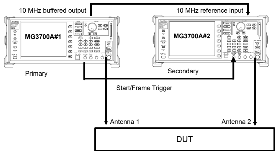
Figure C.1-4 Multiple MG3700A connection (Primary/Secondary)
