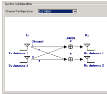
Figure 3.3.5-1 System Configuration ( 2 \times 2 MIMO)
