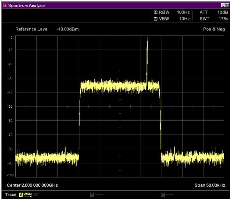
Figure D.1-7 Rice with Flat
