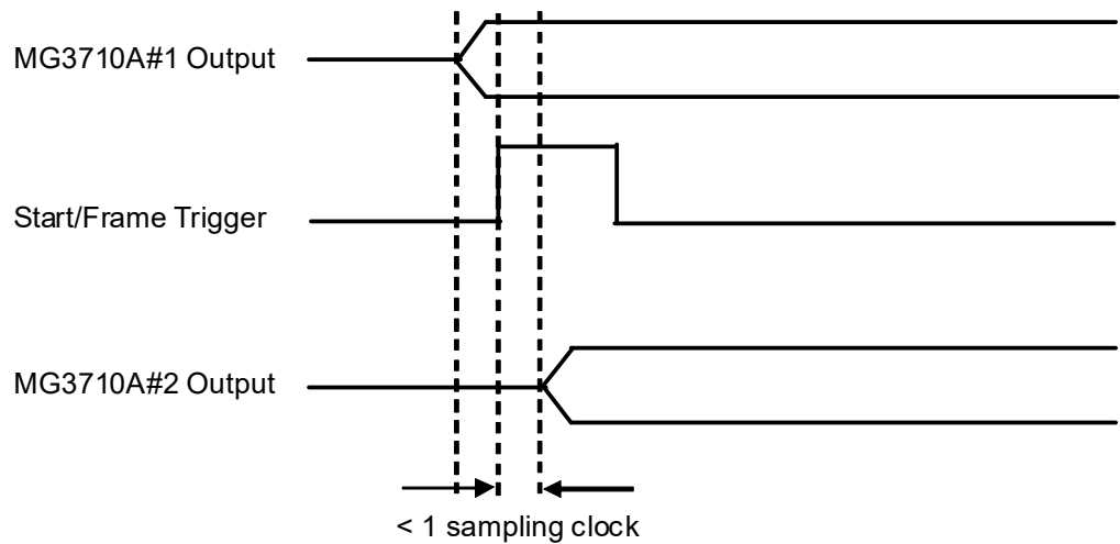
Figure C.2-5 Synchronization relationship of baseband signals when using Primary/Secondary
