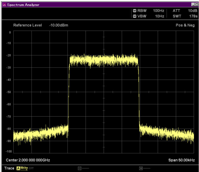
Figure D.1-3 Rayleigh with Flat
