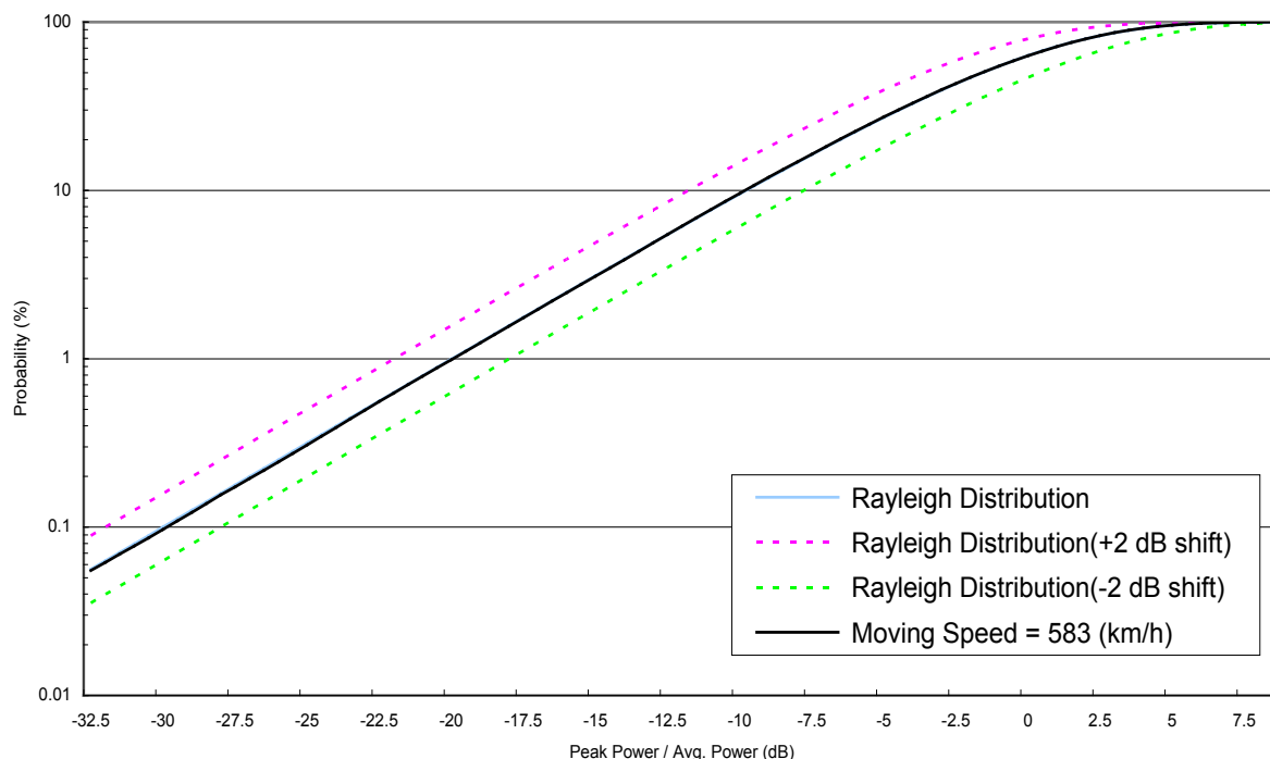
Figure D.2-9 Accumulated probability distribution (Moving Speed = 583 km/h)
