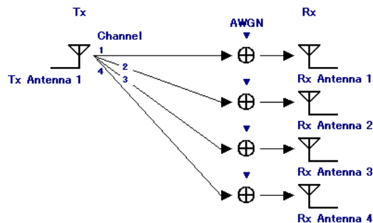
Figure 3.1.2.2-4 1 × 4 SIMO configuration
