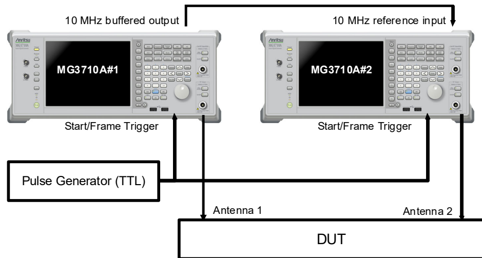
Figure C.2-1 Multiple MG3710A connection (external Start/Frame Trigger)
