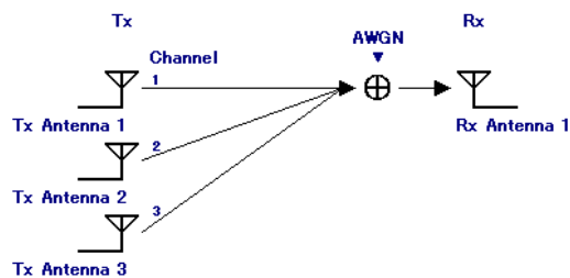
Figure 3.1.2.2-9 3 \times 1 MISO configuration
