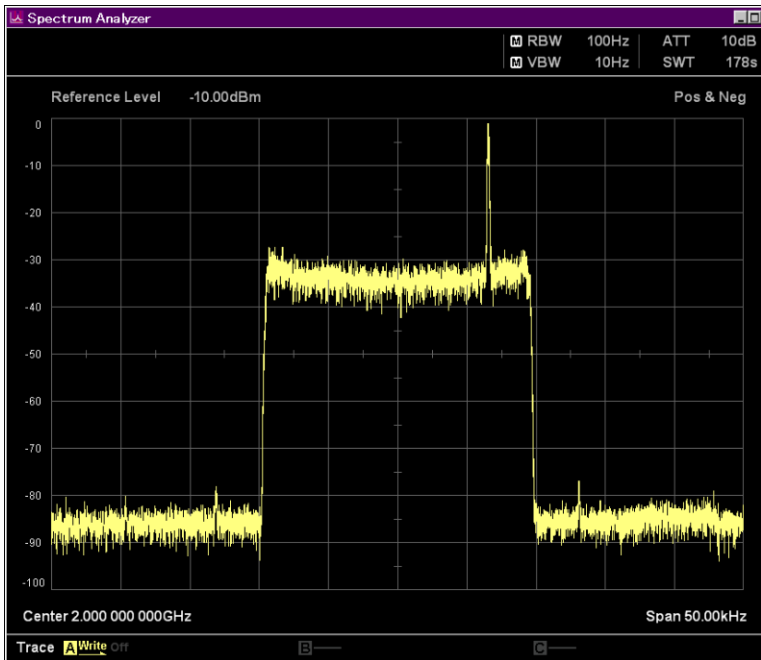
Figure D.1-5 Rice with Classical 3 dB
