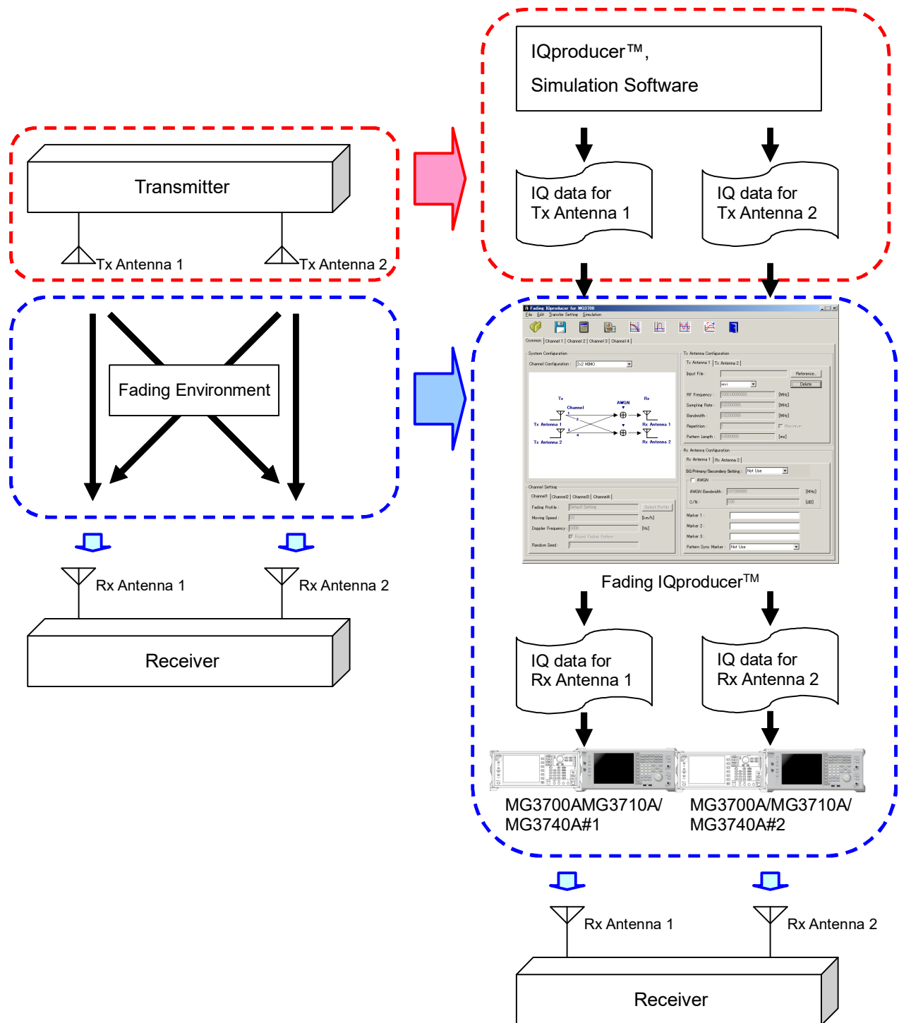
Fig. 1.1-2 2 x 2 MIMO configuration example
