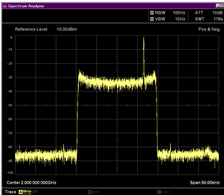
Figure D.1-6 Rice with Classical 6 dB
