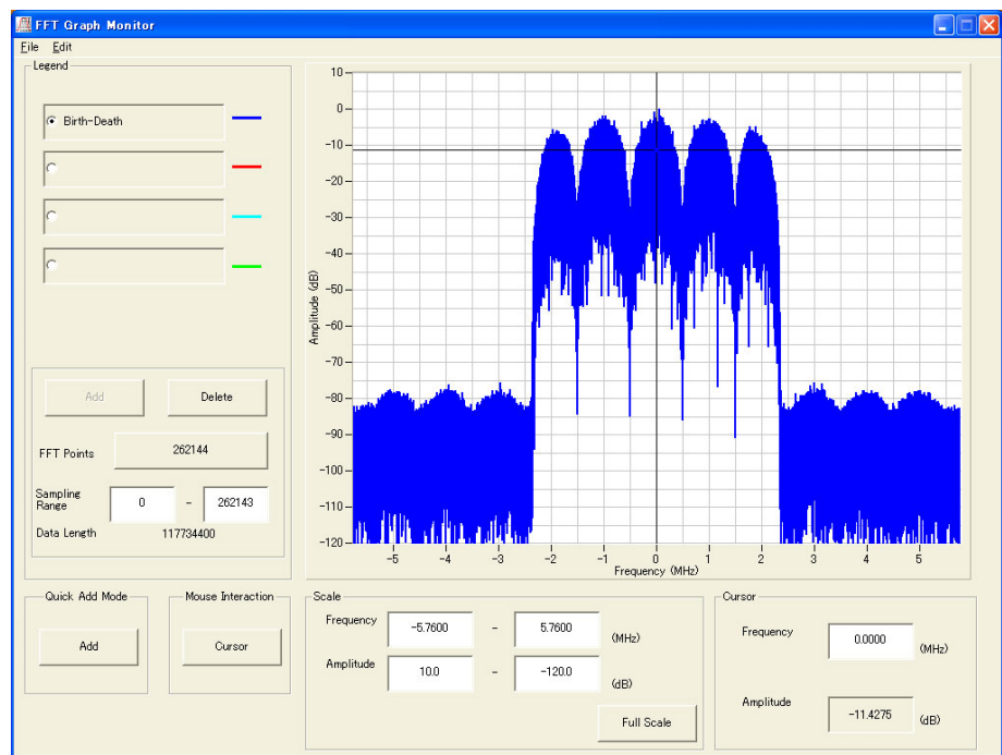
Figure 3.3.3-10 Spectrum (Birth-Death Propagation)
