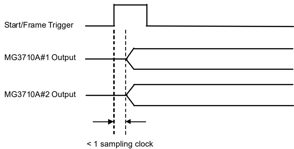
Figure C.2-2 Synchronization-baseband signals when using external Start/Frame Trigger
