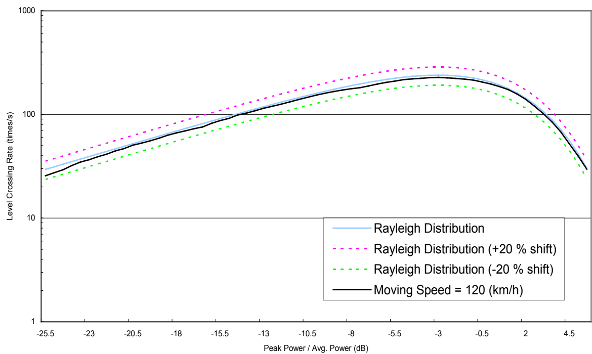
Figure D.2-6 Level crossing rate (Moving Speed = 120 km/h)
