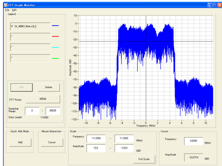
Figure 3.3.5-14 Spectrum (Rx Antenna 2)
