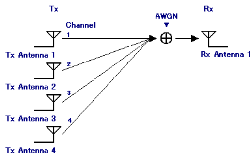
Figure 3.1.2.2-13 4 \times 1 MISO configuration
