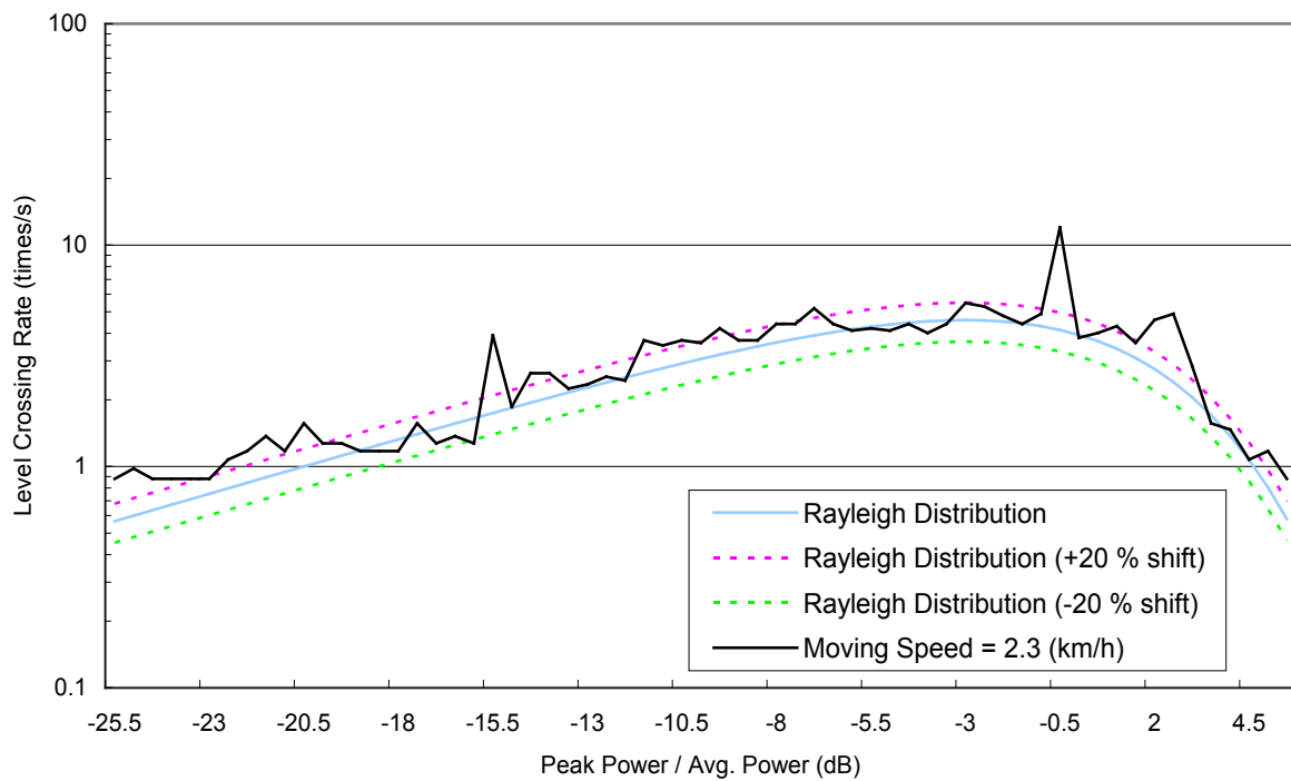
Figure D.2-2 Level crossing rate (Moving Speed = 2.3 km/h)
