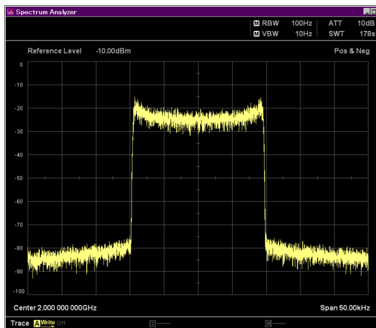
Figure D.1-2 Rayleigh with Classical 6 dB
