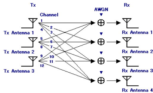
Figure 3.1.2.2-12 3 \times 4 MIMO configuration
