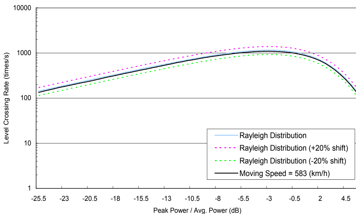
Figure D.2-10 Level crossing rate (Moving Speed = 583 km/h)
