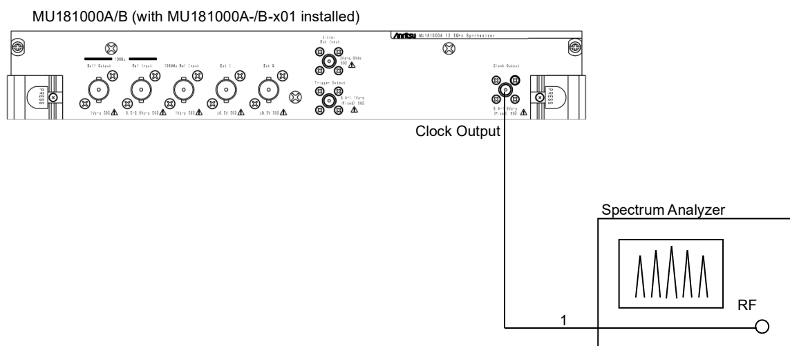
Figure 6.3.3-1 Connection diagram for internal sine wave jitter measurement of 0.4 Ulp-p or less
