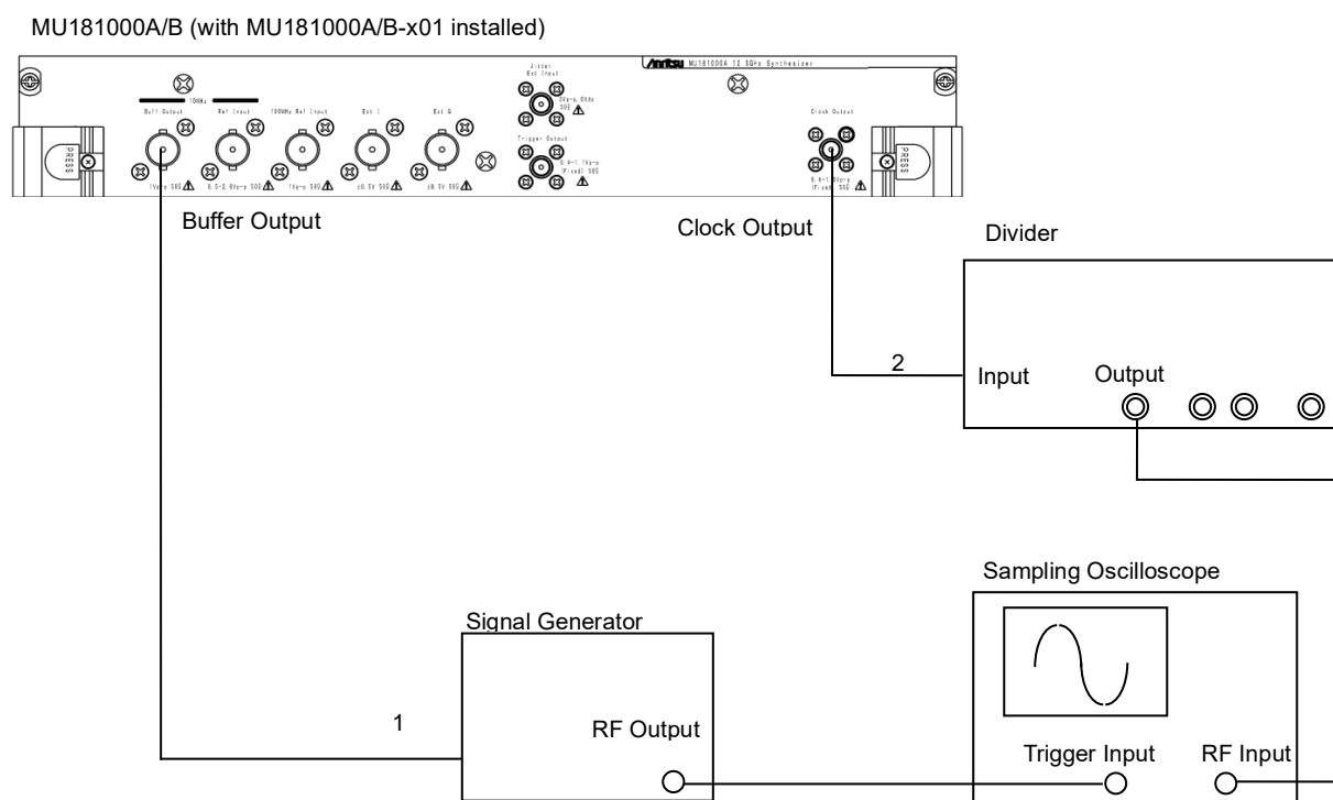
Figure 6.3.5-1 Connection diagram for triangular wave modulation measurement
