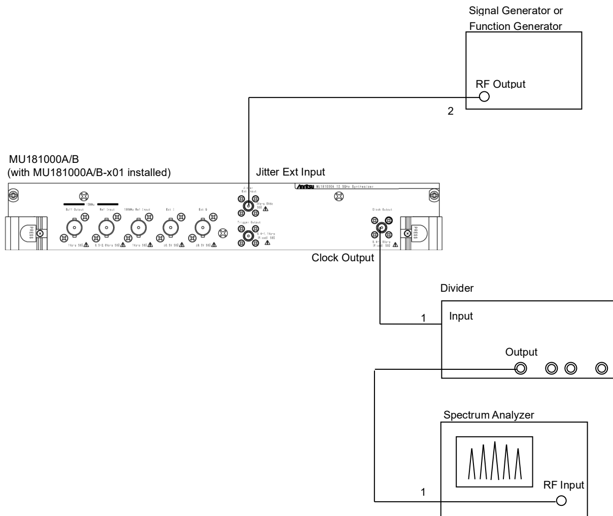
Figure 6.3.4-2 Connection diagram for external sine wave jitter measurement of more than 0.4 Ulp-p
