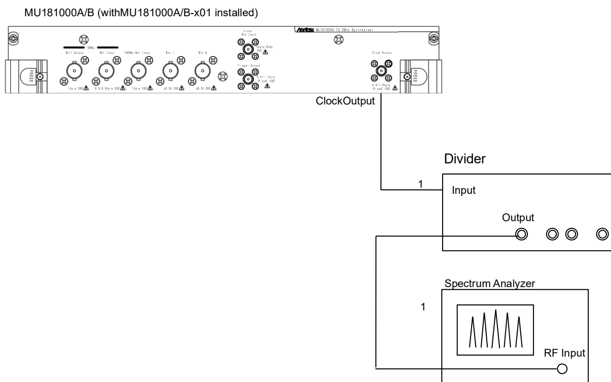
Figure 6.3.3-2 Connection diagram for internal sine wave jitter measurement of more than 0.4 Ulp-p
