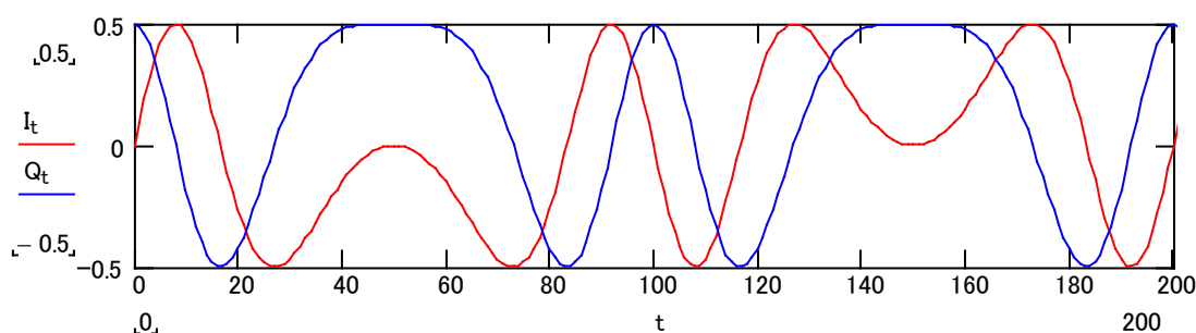
Figure 5.1.2-2 Example of waveforms of I and Q signals when jitter amplitude is 2 UIp-p
