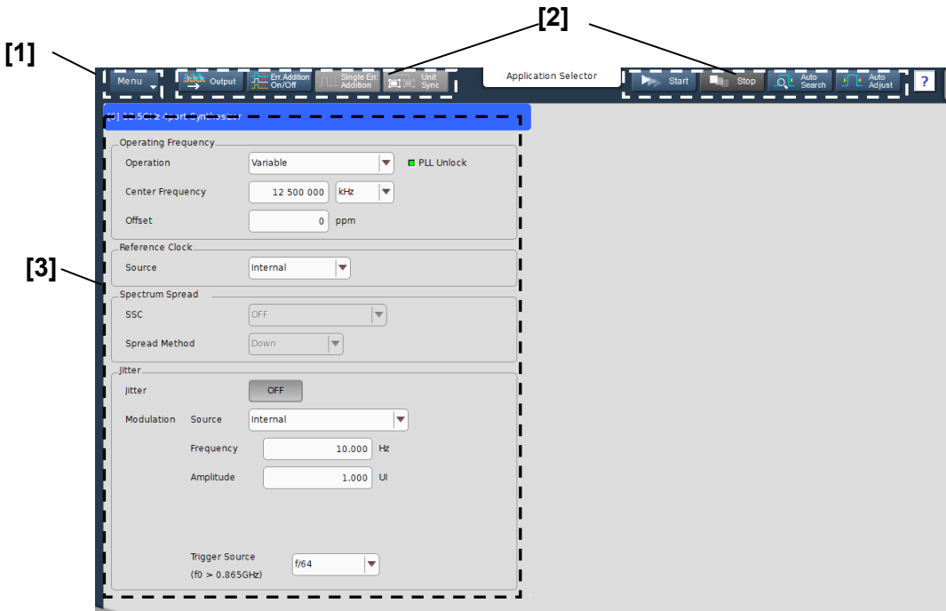
Figure 4.1-2 Configuration of entire setup dialog box for MU181000A/B (MP1900A)
