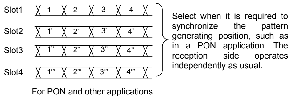
Figure 5.5.1-4 Channel Synchronization pattern generation/reception
