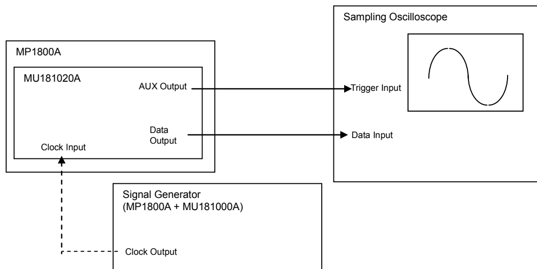
Figure 7.3.2-1 Connection diagram for waveform test
