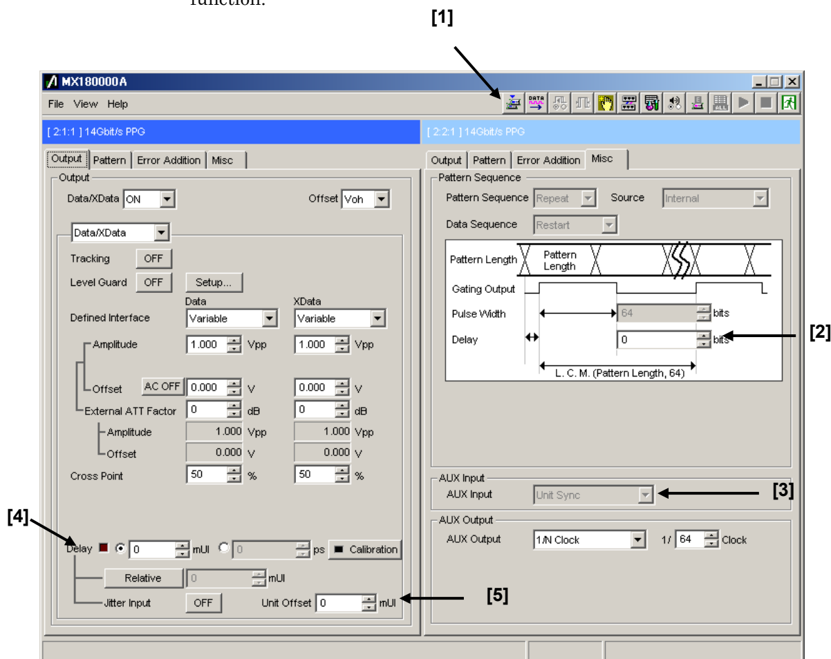
Figure 5.6.3-1 MX180000A Screen
