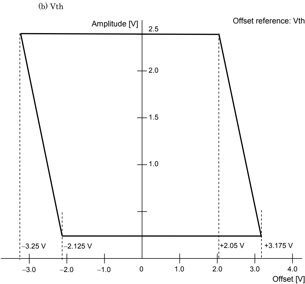
Figure C.1.1.2-2 Setting range of amplitude and offset based on offset reference ( V_{th} ) (MU181020A/B -x11)
