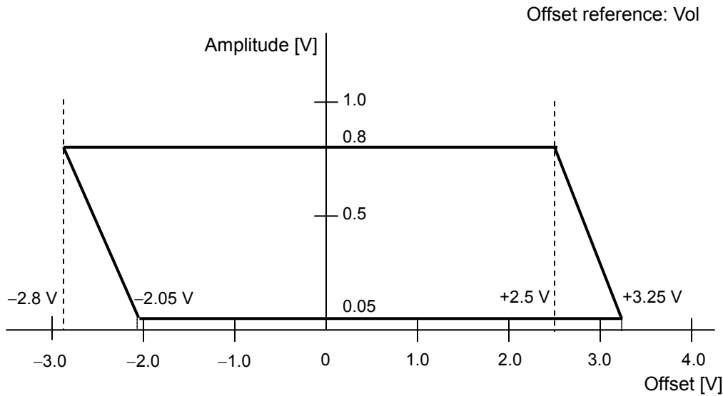
Figure C.1.1.1-3 Setting range of amplitude and offset based on offset reference (Vol) (MU181020A-x10)
