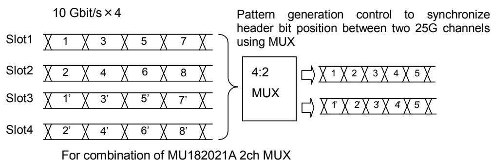
Figure 5.5.1-6 25G Channel Synchronization pattern generation/reception
