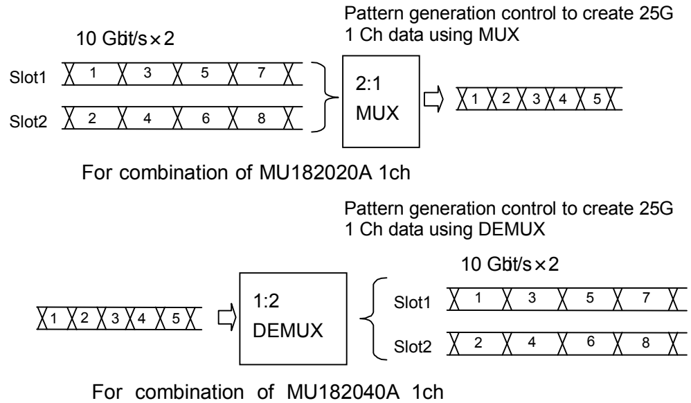
Figure 5.5.1-3 2ch Combination pattern generation/reception
