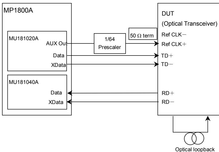
Figure 6.1.1-1 Connection diagram for XFP module evaluation
