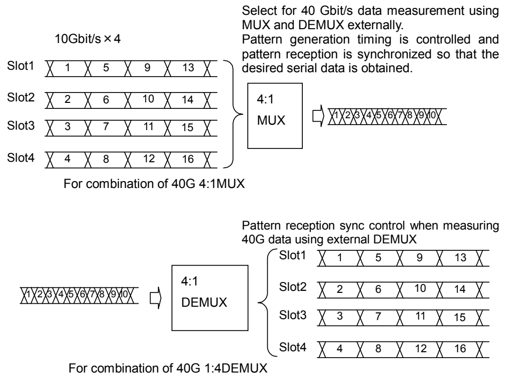
Figure 5.5.1-1 4ch Combination pattern generation/reception
