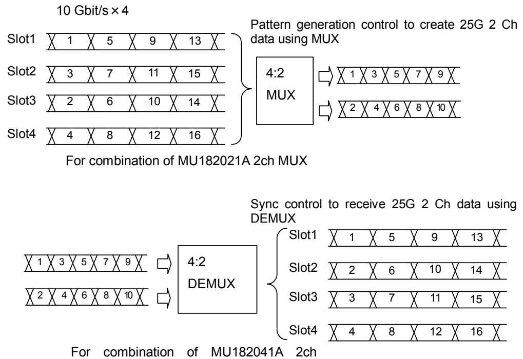
Figure 5.5.1-2 25Gx2ch Combination pattern generation/reception
