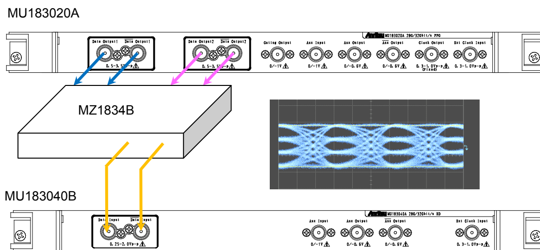
Figure G.1-1 PAM Signal and Connection Example for BER Measurement
