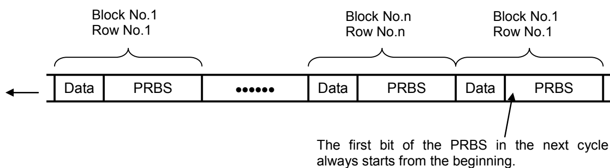
Figure 5.2.5-3 Continuity of PRBS pattern strings (Restart)
