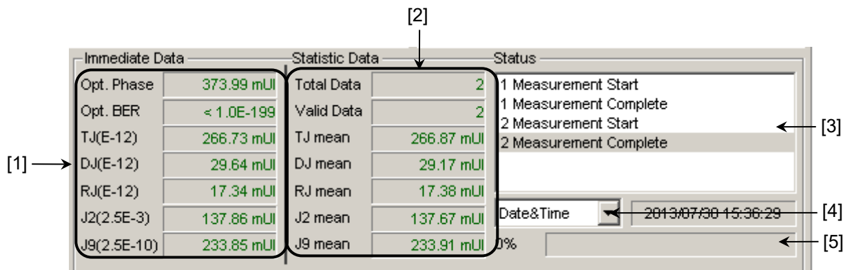
Figure 5.12.1.4-1 Measurement result display area
