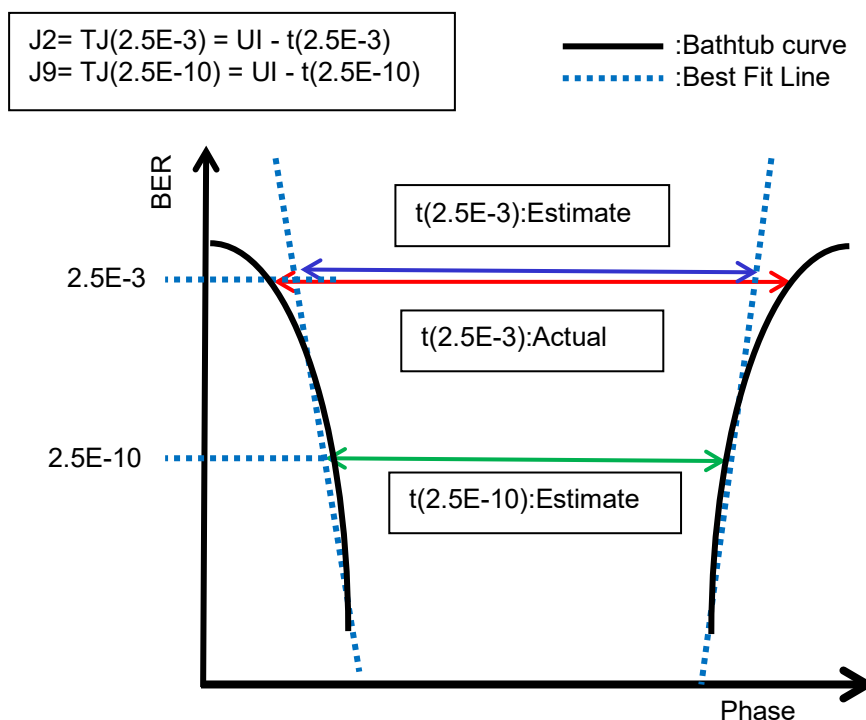
Figure 5.12.1.2-4 J2 Calculation
