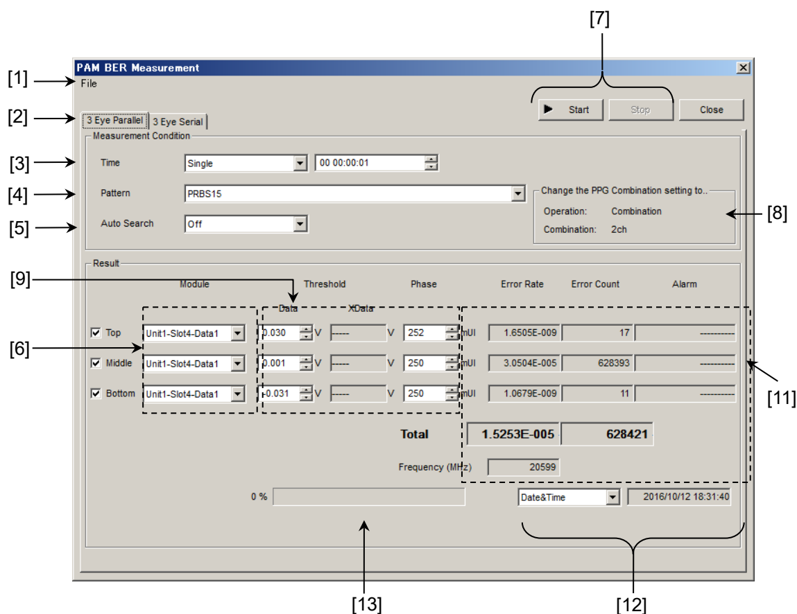
Figure 5.14.1-2 PAM BER Measurement window (3 Eye Parallel mode)
