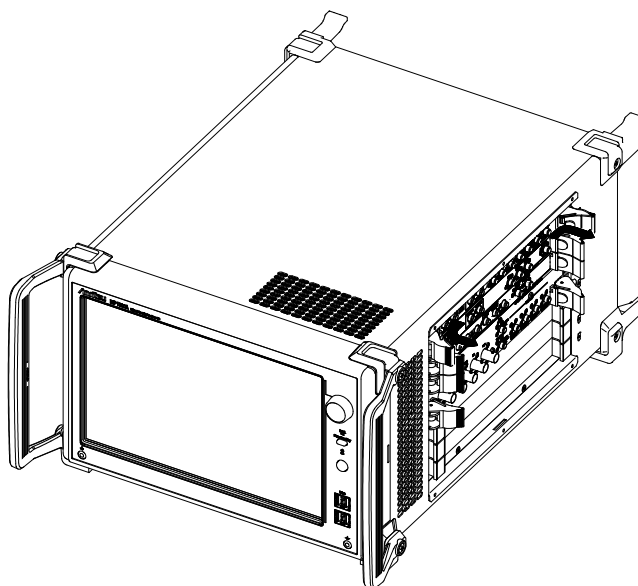
Figure 3.3.2-2 Modules ejectors
