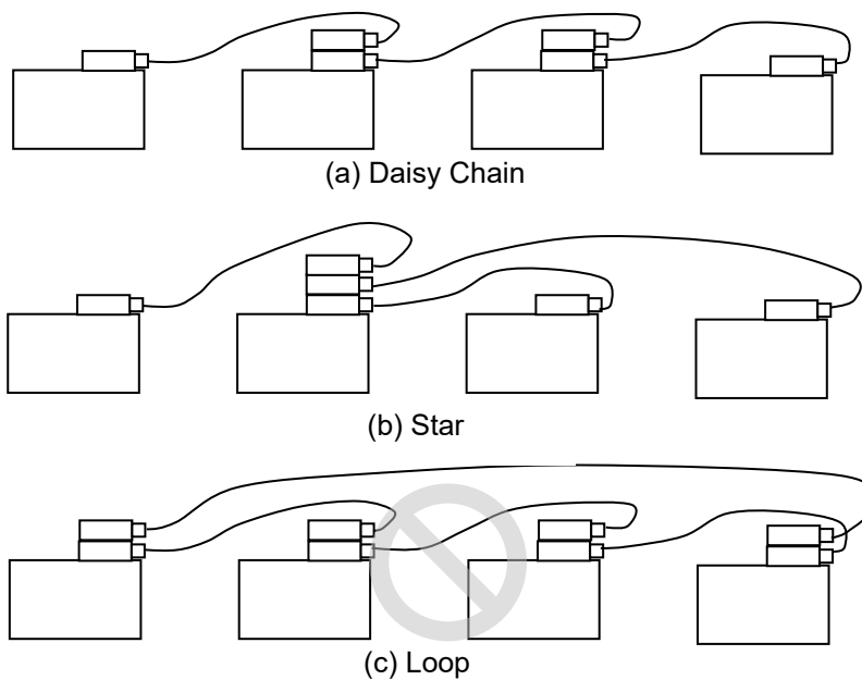
Figure 5.3-2 GPIB Cable Connection Methods
