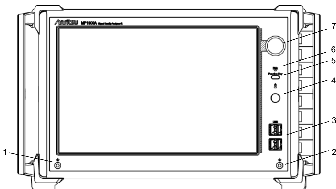
Figure 2.1-1 Front panel
