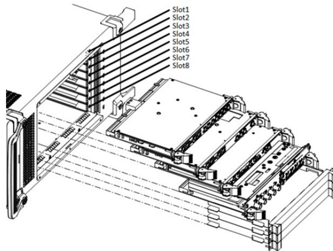
Figure 3.3-1 MP1900A modules
