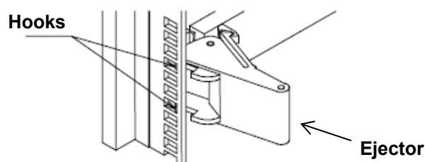
Figure 3.3.1-1 Module hooks
