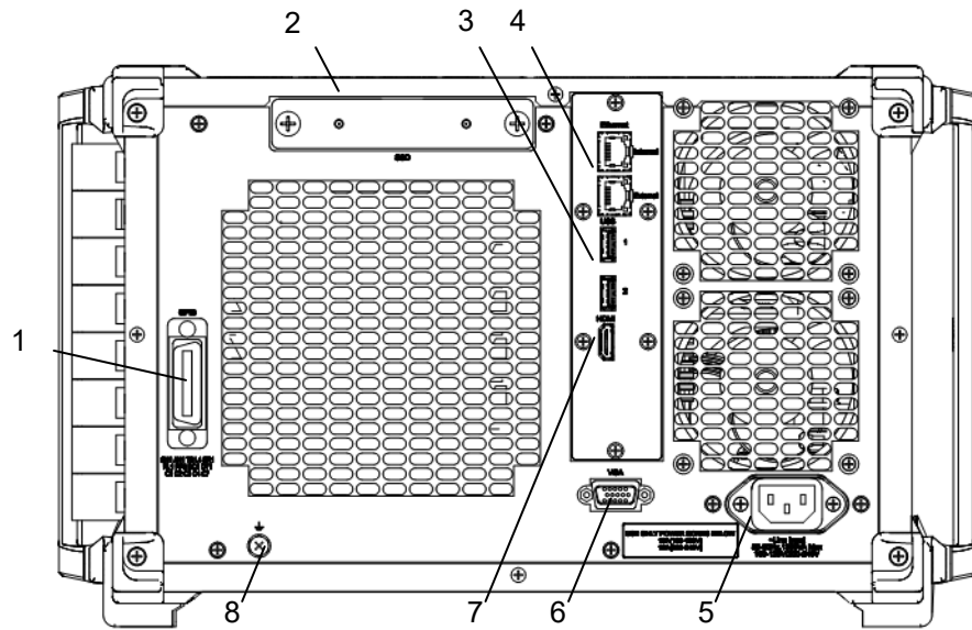
Figure 2.2-1 Rear panel
