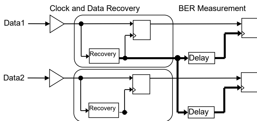
Figure 5.14.1-6 Clock and Data Recovery Circuit
