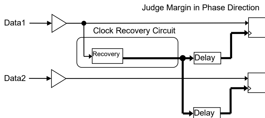
Figure 5.14.1-5 Recovered Clock Circuit
