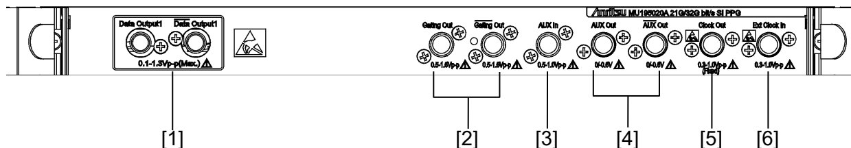
Figure 3.1.1-1 Panel layout (MU195020A-x10)
