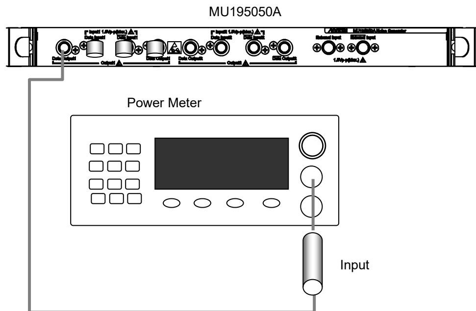
Figure 8.3.6-1 Connection for CMI/DMI Test
