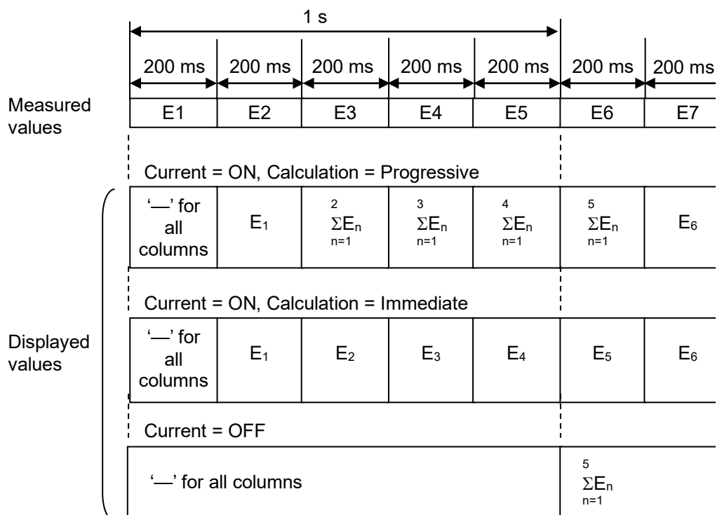
Figure 5.11.2-4 Relationship between measured values and displayed values
