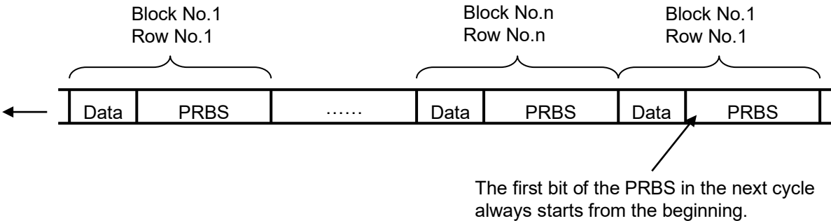
Figure 5.3.5-2 Continuity of PRBS pattern strings (Restart)
