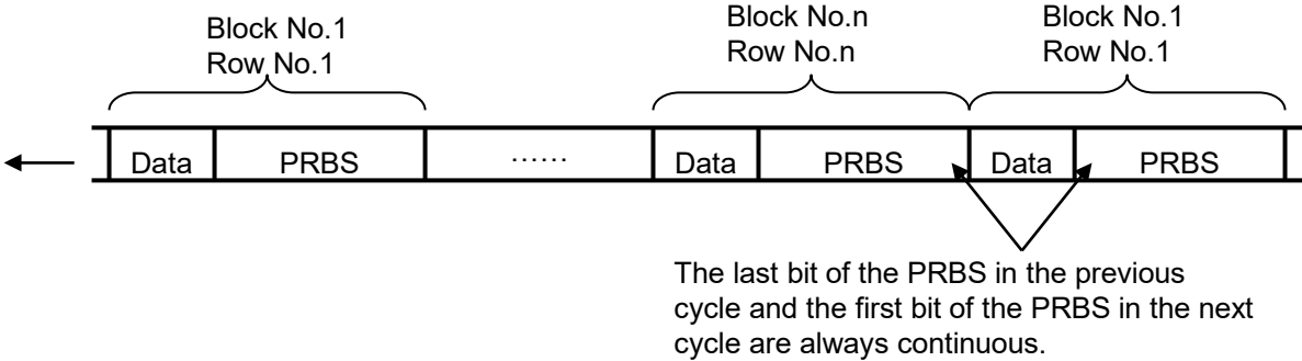
Figure 5.3.5-3 Continuity of PRBS pattern strings (Consecutive)
