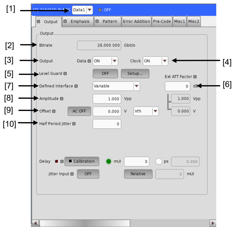
Figure 5.1.1-1 Output Tab
