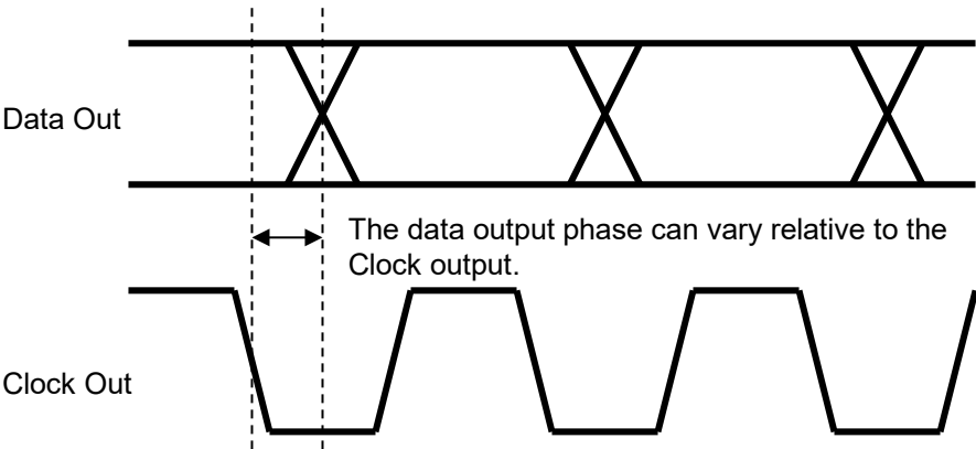
Figure 5.1.2-1 Delay Setting
