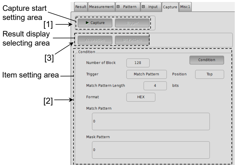
Figure 5.15.1-1 Capture Tab
