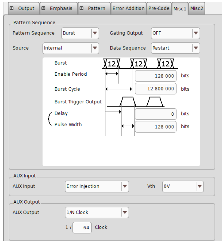
Figure 5.6-1 Misc1 Tab
