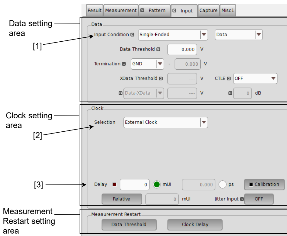
Figure 5.14.1-1 Input Tab
