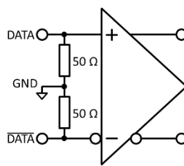
Termination GND
