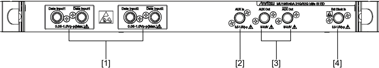
Figure 3.1.2-2 Panel Layout (MU195040A-x20)
