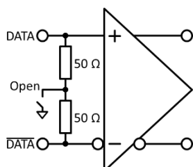
Differential 100 \Omega
