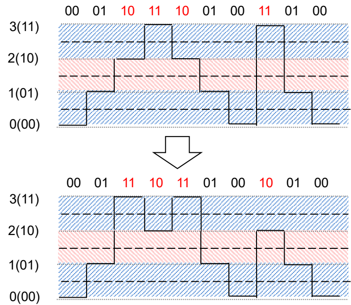
Figure 5.3.6-4 Gray Coding PAM4 Pattern Waveform
