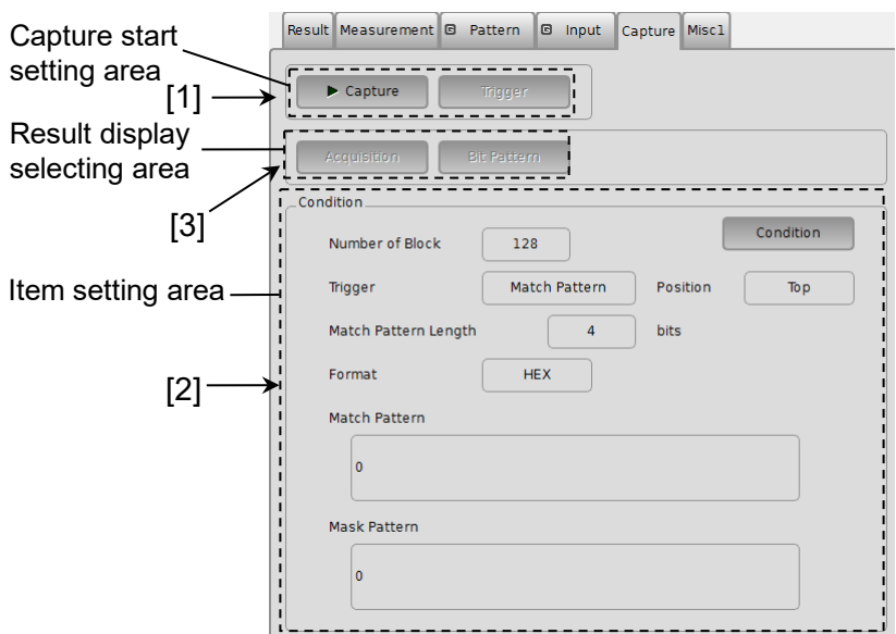
Figure 5.15.1-1 Capture Tab
