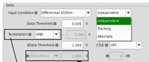
Differential input setting window (Termination: 50 \Omega )
