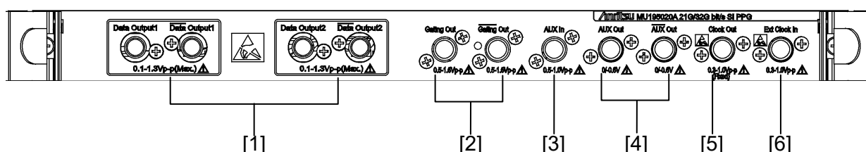
Figure 3.1.1-2 Panel layout (MU195020A-x20)
