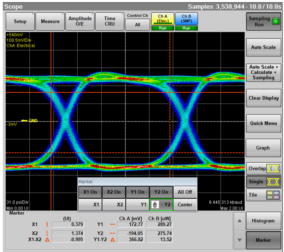
Figure 6.9.5-1 Marker Display
