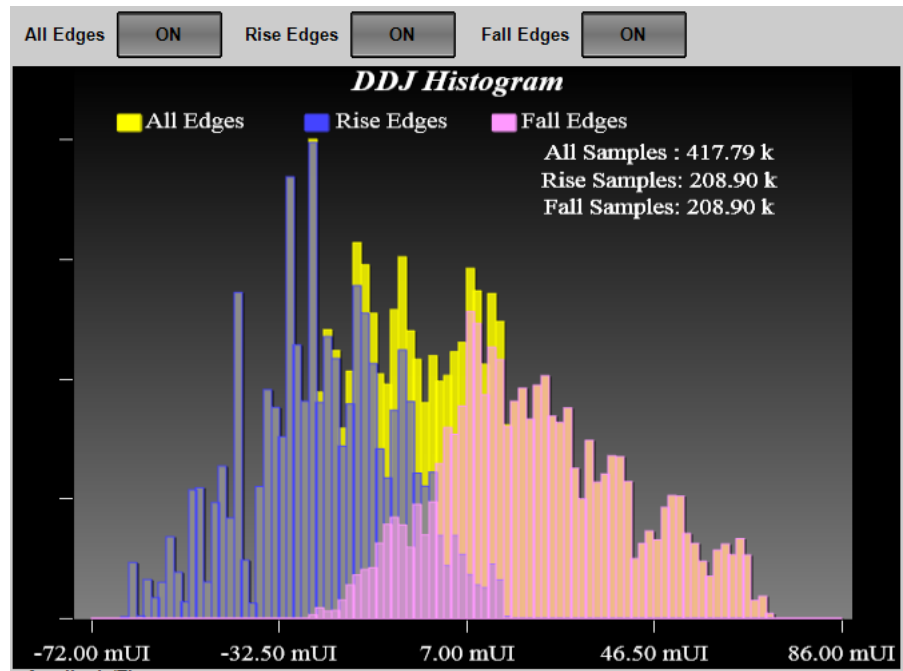
Figure 6.2.2.2-5 DDJ Histogram
