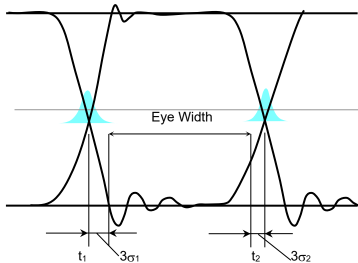
Figure 1.5-16 Eye Width
