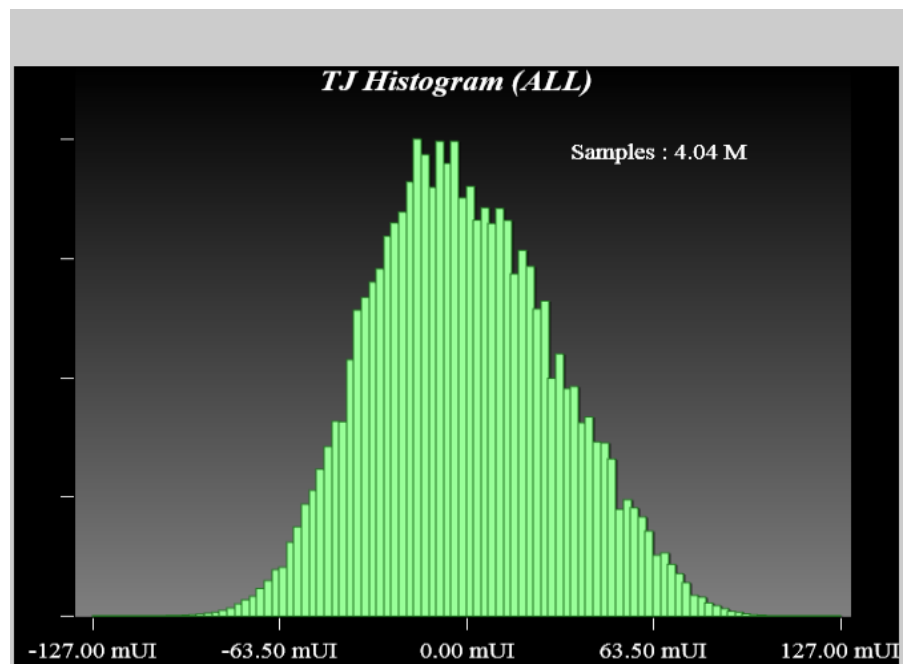
Figure 6.2.2.2-1 TJ Histogram
