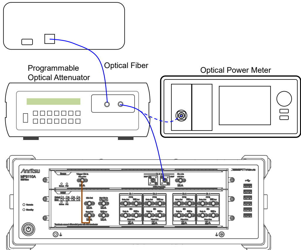
Figure 7.3.3-1 Optical Power Meter Test Connection Diagram (SMF, When using a PPG of MP2110A)
