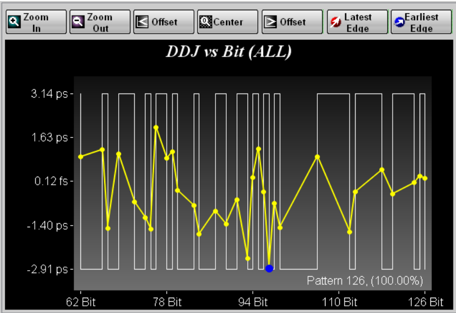
Figure 6.2.1-18 DDJ vs Bit
