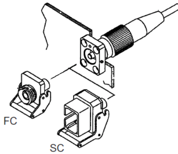
Figure 8.2-1 Connector Type
