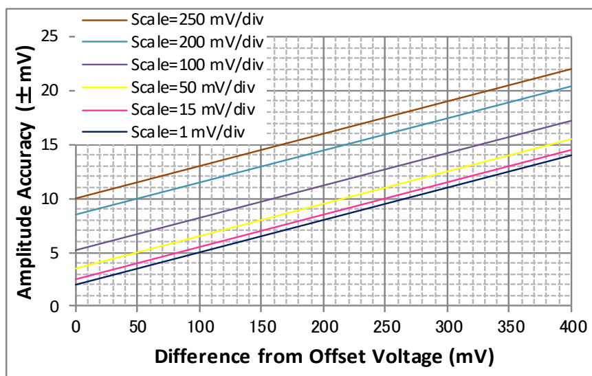
Figure 7.3.2-1 Offset Amplitude Accuracy
