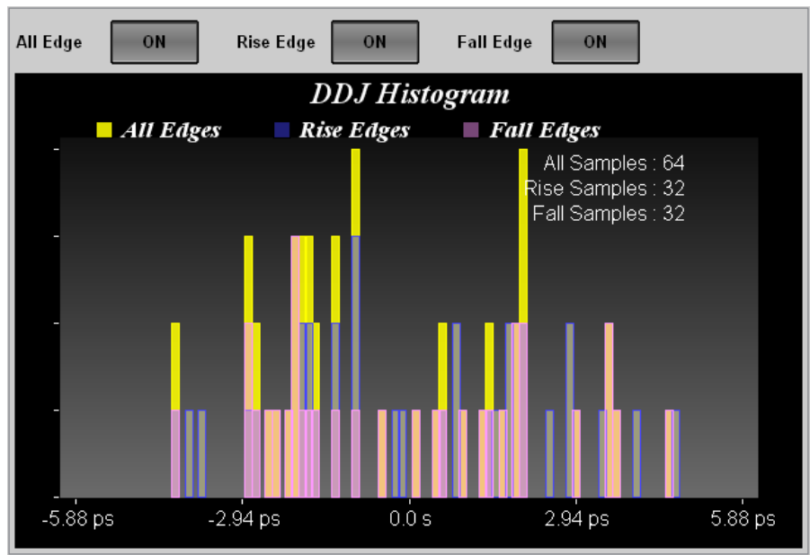
Figure 6.2.1-16 DDJ Histogram
