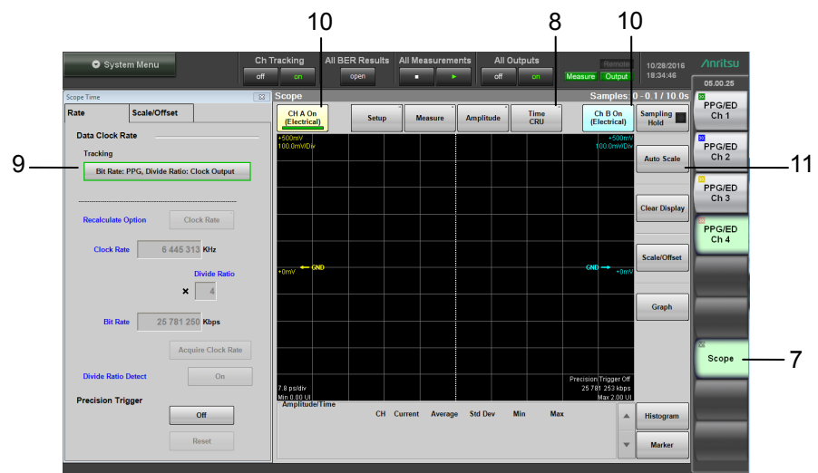
Figure 3.2-3 Scope Operation
