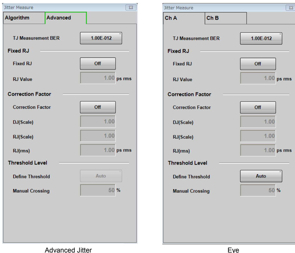
Figure 6.2.3-7 Jitter Measure Dialog Box (Advanced Tab)
