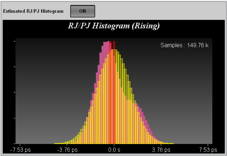
Figure 6.2.1-14 PJ/RJ Histogram
