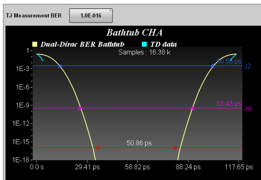
Figure 6.2.1-11 Bathtub CHA
