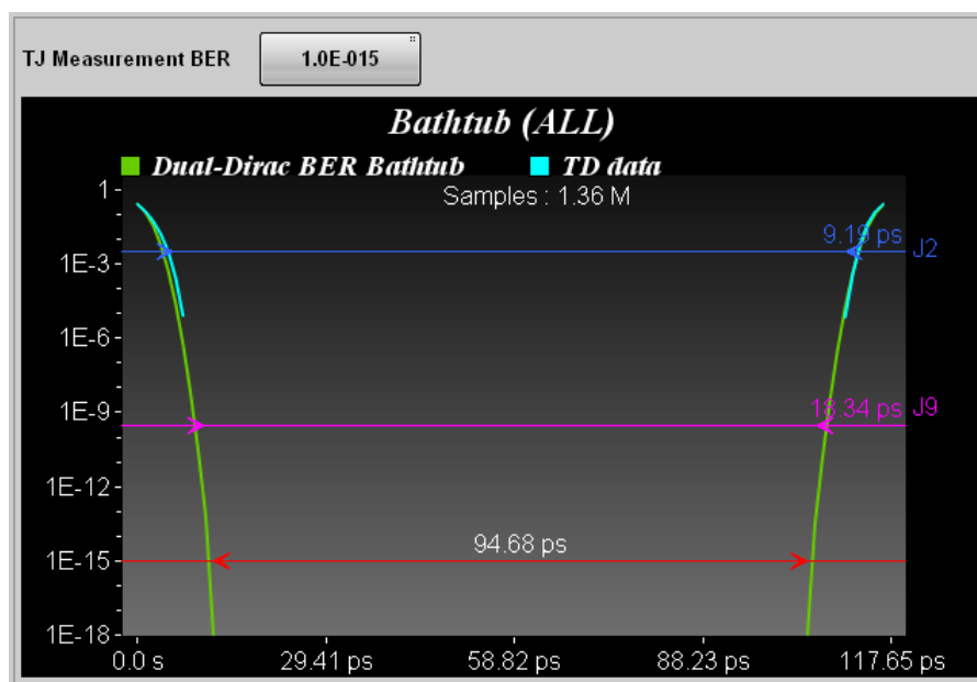
Figure 6.2.1-13 Bathtub
