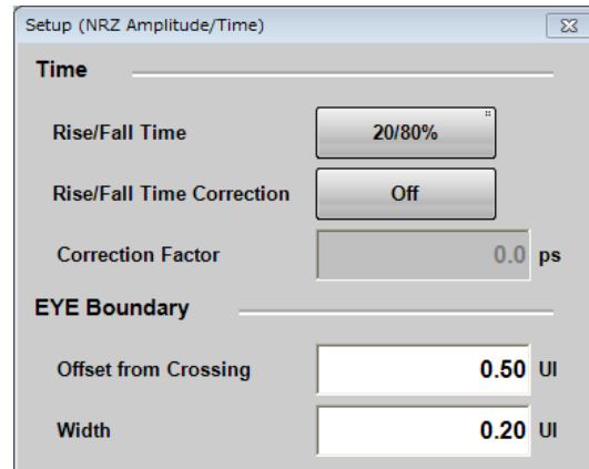
Figure 6.9.1.1-1 Setup (NRZ Amplitude/Time) Dialog Box
