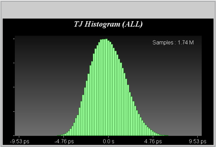
Figure 6.2.1-12 TJ Histogram
