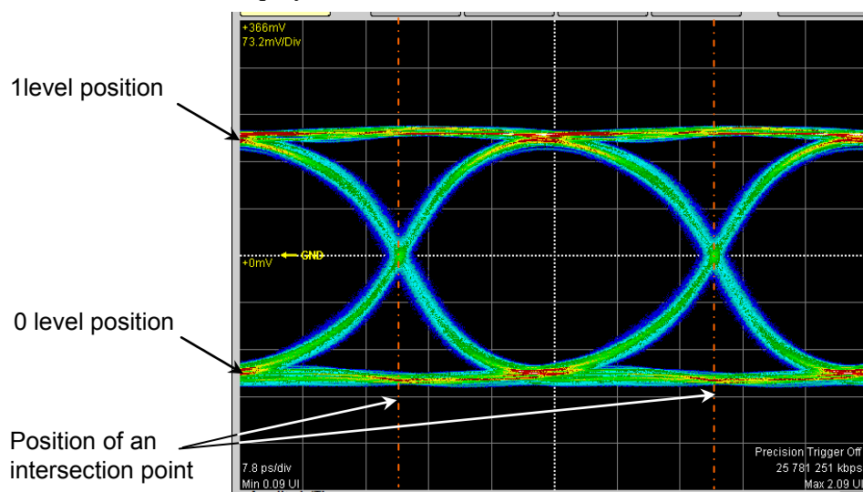
Figure 6.8.1-1 Waveform Display after Auto Scale (Eye/Coherent Eye Mode)
