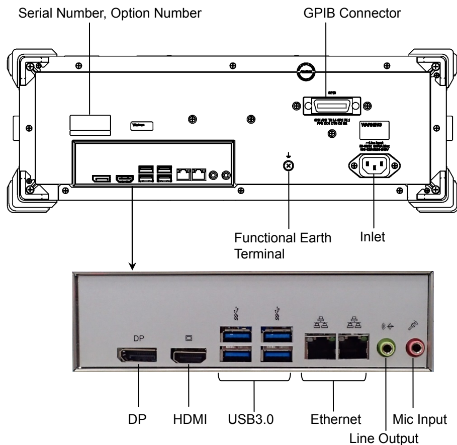
Figure 2.2.2-1 Rear Panel
