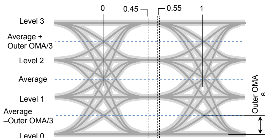
Figure 1.5-26 The position for TDECQ measurement
