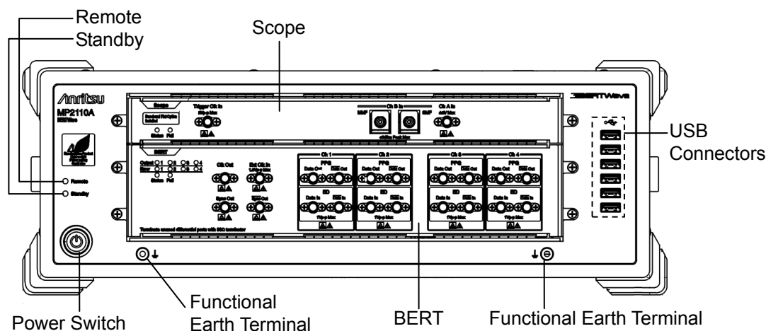
Figure 2.2.1-1 Front Panel
