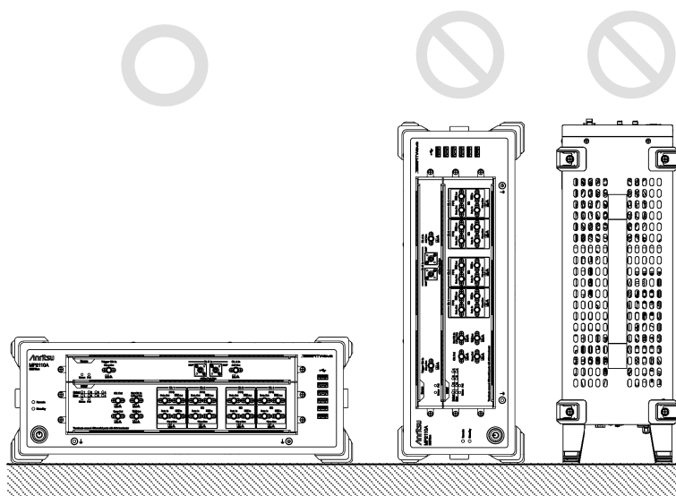
Figure 2.1.2-1 Installation Orientation
