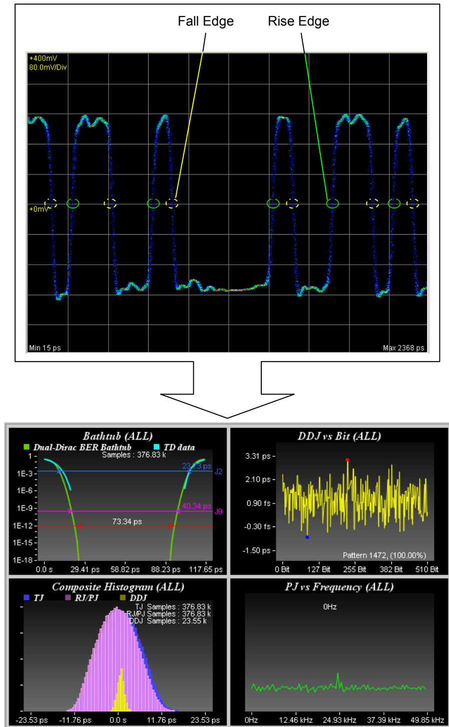
Figure 6.9.3-3 Measured Part and Display Example of Jitter Analysis (Advanced Jitter)
