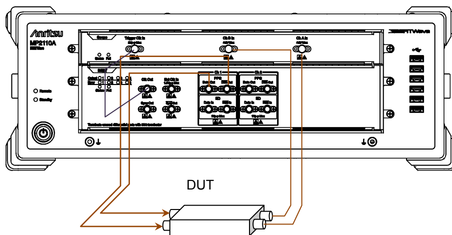
Figure 3.2-1 Electrical Signal Used for DUT Input/Output (MP2110A-012, 021)
