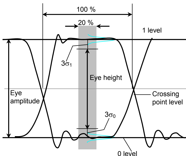
Figure 1.5-21 0 Level, 1 Level, Eye Amplitude and Eye Height
