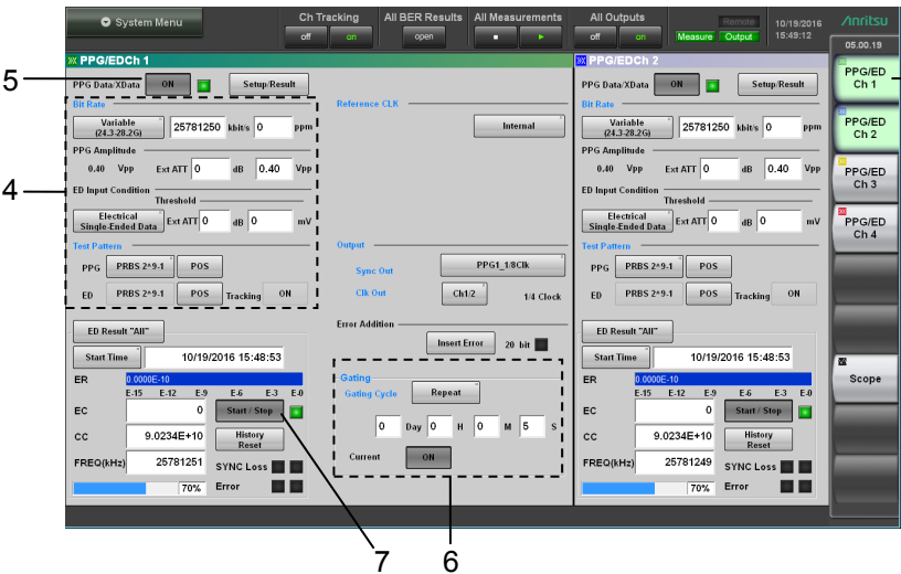
Figure 3.1-2 Operating Bit Error Rate Measurement
