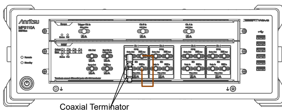
Figure 7.2.4-2 ED1 Data In Pattern Test Connection Diagram
