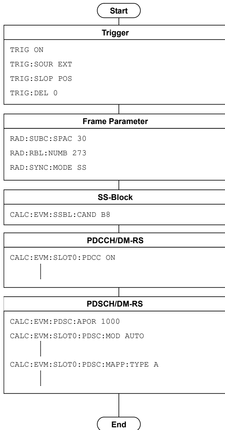
Figure 1.2.3-1 Flow of Common Settings for Modulation and Command Example
