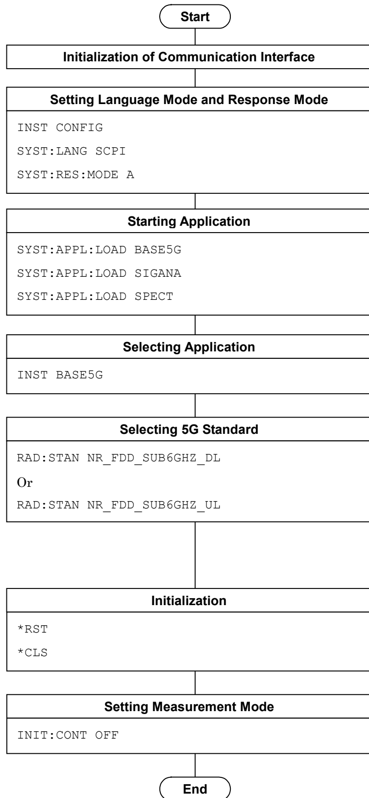
Figure 1.2.1-1 Initialization Flow and Command Example
