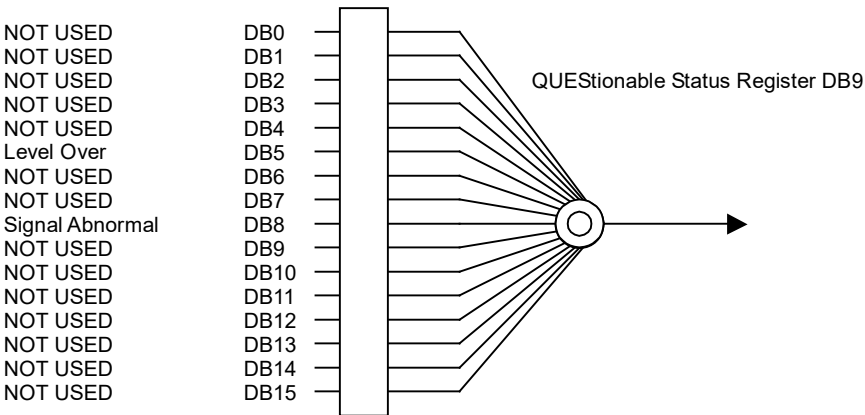
Figure 3.2-2 QUEStionable Measure Register
