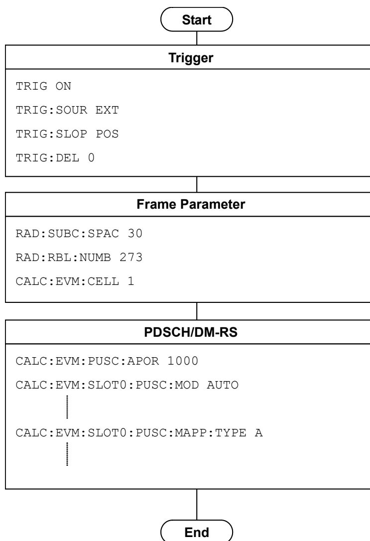
Figure 1.2.3-2 Flow of Common Settings for Modulation and Command Example
