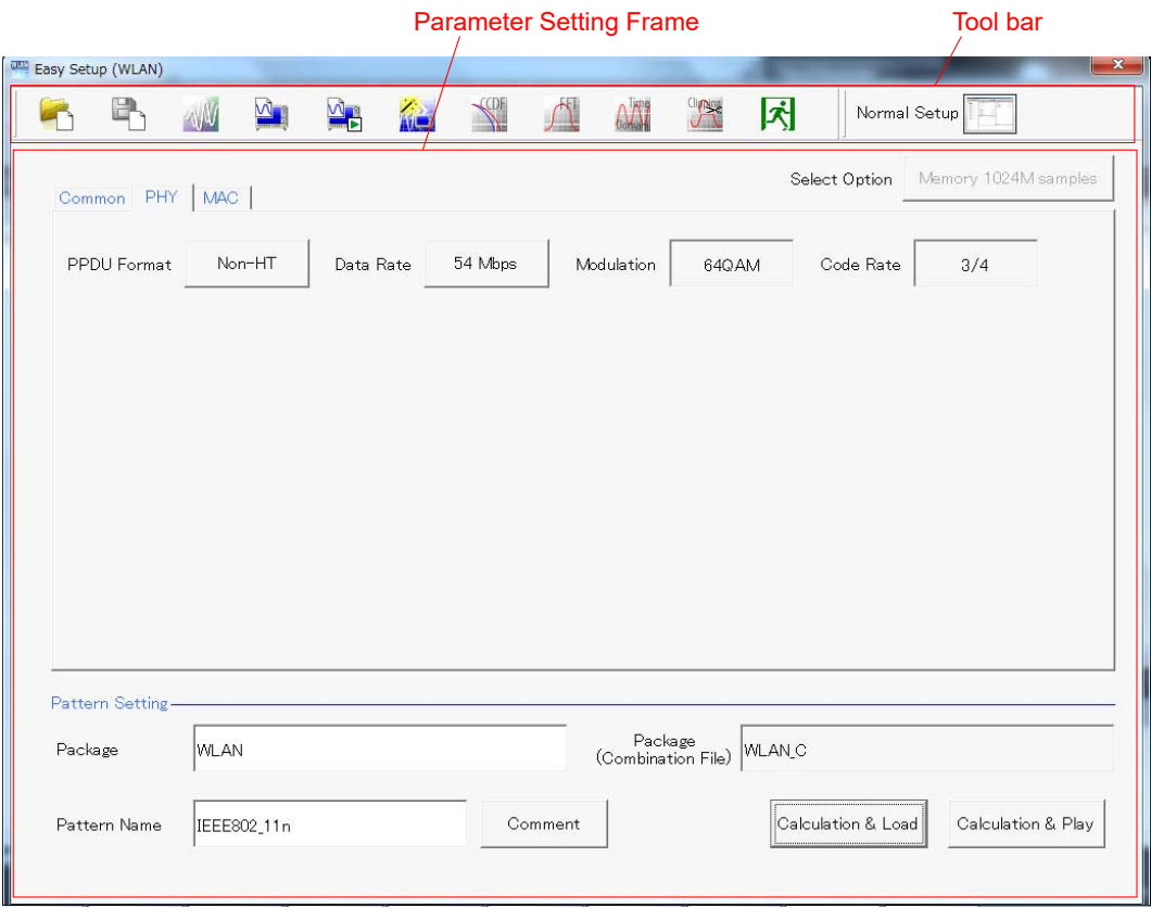
Figure 4.2.10-3 PHY Tab (When System is Set to 11n and PPDU Format is Set to Non-HT)
