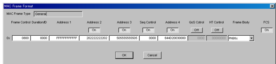
Figure 3.1.4.4-1 MAC Frame Format setting window (System = 11ac)
