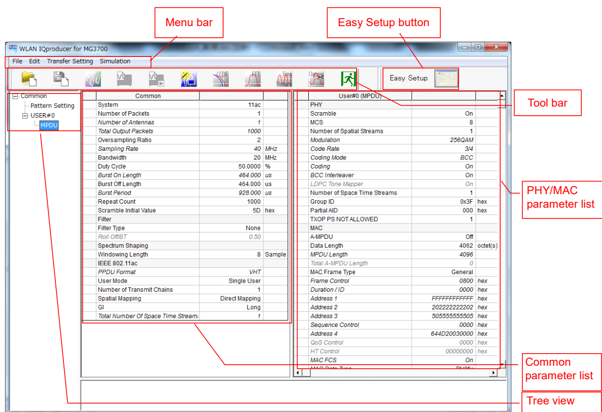
Figure 3.1.1-2 Main screen (11ac)
