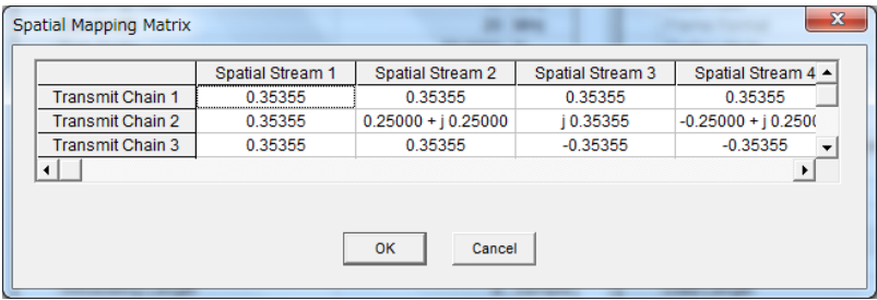
Figure 3.1.3.2-2 Spatial Mapping Matrix Setting Window (Number of Transmit Chains= 8)
