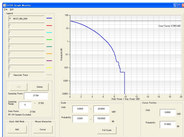
Figure 3.5-1 CCDF Graph Monitor screen
