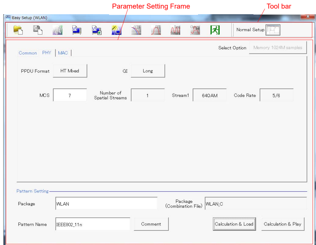
Figure 4.2.10-2 PHY Tab (When System is Set to 11n and PPDU Format is Set to HT Mixed or HT-GreenField)
