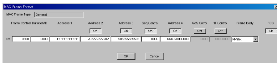
Figure 3.1.4.2-1 MAC Frame Format setting window (when System = 11n)
