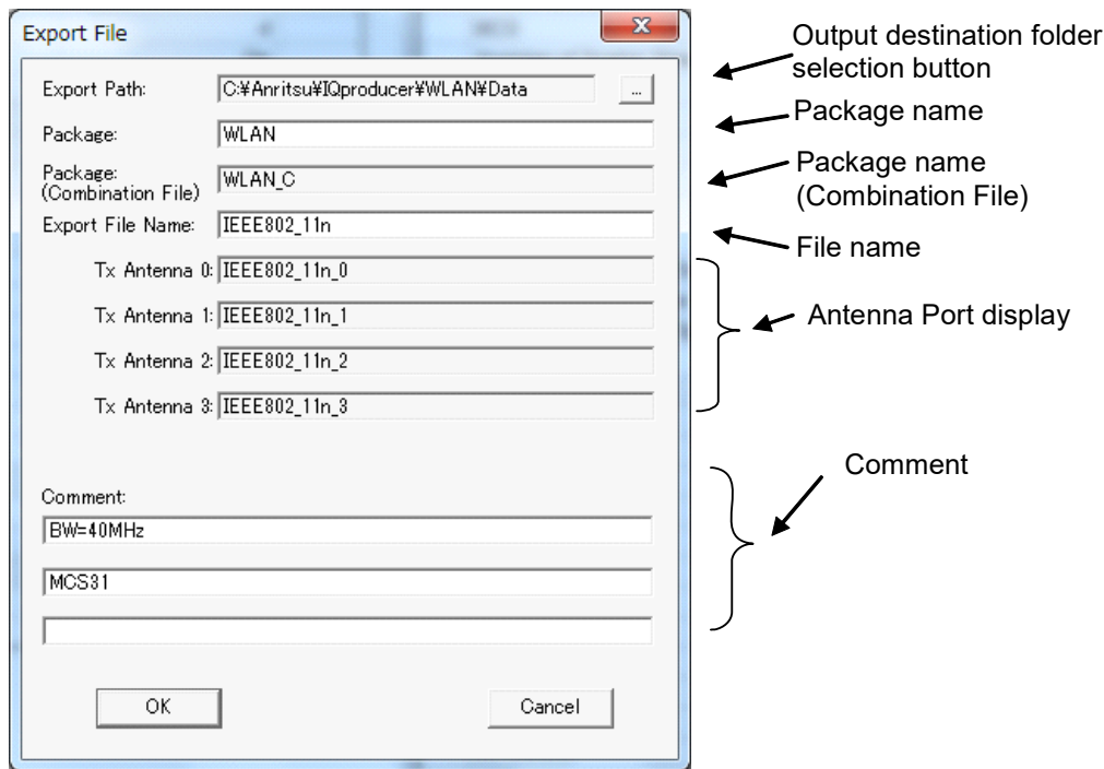
Figure 3.1.5-3 Export File screen (when Number of Antennas = 4)
