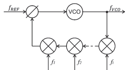
Figure 6 Consecutive frequency conversion within phase-lock loop
