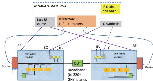
Figure 2 The block diagram of the 220+ GHz broadband VNA is shown here. Multiplexing is used on both stimulus (A-D are different multipliers for the different sub-bands) and receivers.
