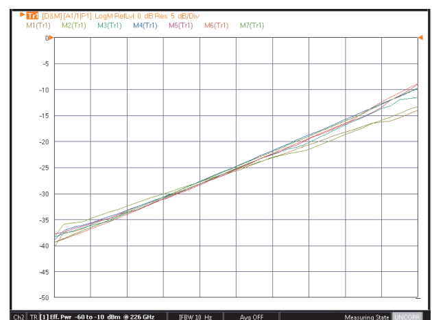
Figure 5 Power sweeps at a number of frequencies up to 226 GHz illustrate the power control range.
