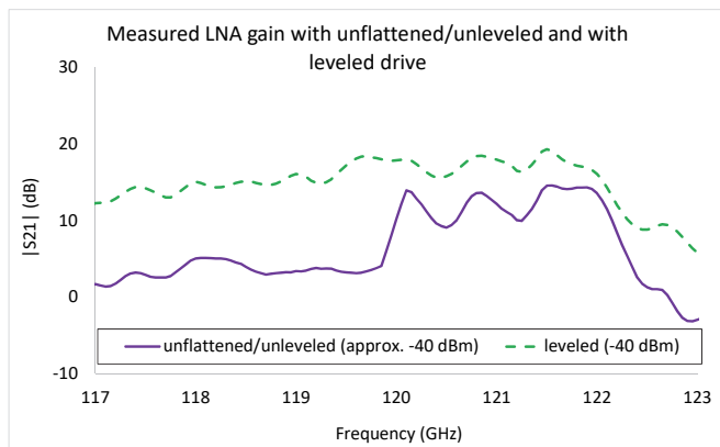
Figure 1 The effects of an unflattened/unleveled stimulus on a mm-wave LNA measurement can be substantial. Isolated transistor measurements can be more affected.
