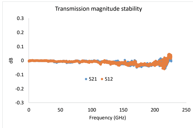
Figure 3 Stability and trace noise are important metrics of S-parameter data usability for modeling and characterization.
