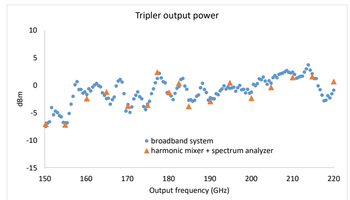
Figure 8 Multiplier output as measured with the current system (with higher point count and absolute receiver calibrations) and with a harmonic mixer/spectrum analyzer pair with padding and additional calibrations showed decent agreement.
