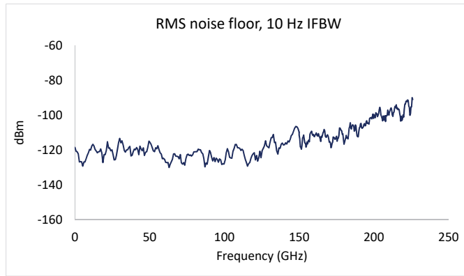
Figure 6 Instrument noise floor can be important when device stimulus levels must be very low.
