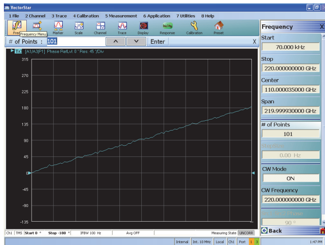
Figure 7 A dual-source drive with controlled phase relationship is needed for true differential drive and related measurement requirements.
