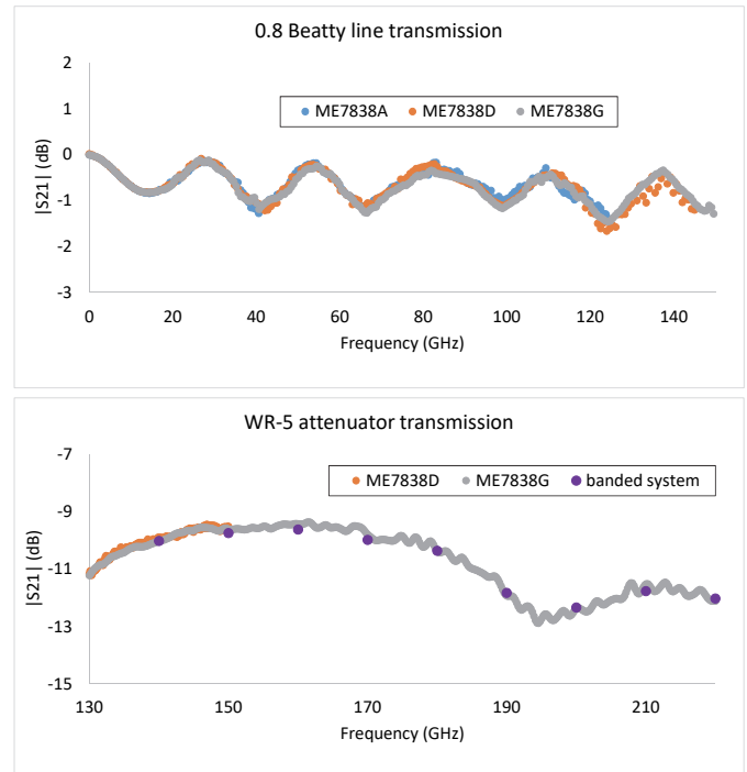
Figure 4 Calibrated measurements (using coaxial and waveguide calibration kits) of artifacts offer a basis of comparison between systems
