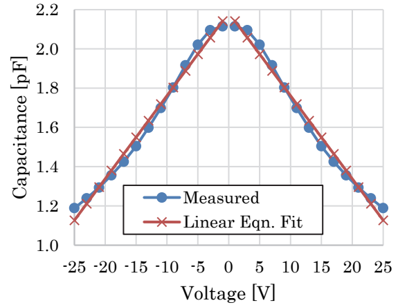
Figure 7 Capacitance vs. Voltage, Measured and Linear Eqn. Fit (Tecdia PN: HBC2R2KY20X10X5A02)
