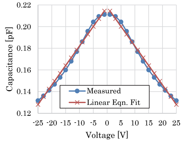
Figure 6 Capacitance vs. Voltage, Measured and Linear Eqn. Fit (Tecdia PN: HBCR22AY20X10X5A02)
