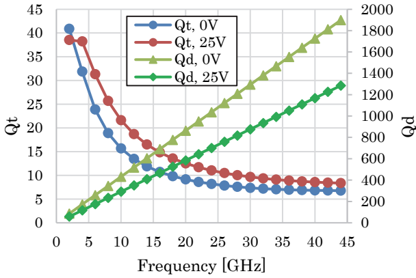
Figure 4 Q_t and Q_d vs Frequency vs. applied voltage (Tecdia PN: HBCR22AY20X10X5A02)
