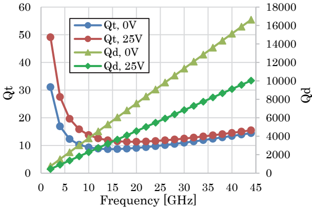
Figure 5 Q_t and Q_d vs Frequency vs. applied voltage (Tecdia PN: HBC2R2KY20X10X5A02)
