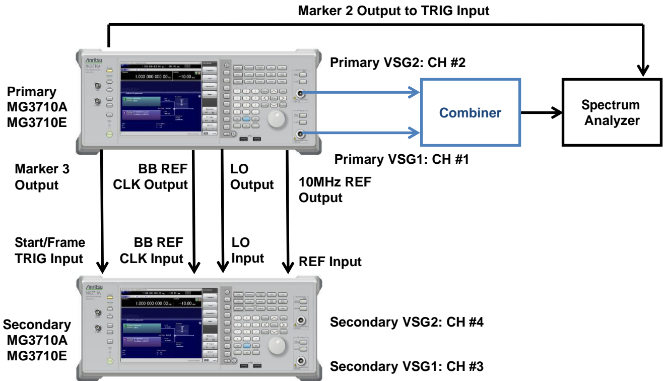
Figure 12. 4x4 MIMO configuration (Connection between Combiner and Spectrum Analyzer is for adjustment to VSG1 and VSG2 in primary MG3710A / MG3710E)
