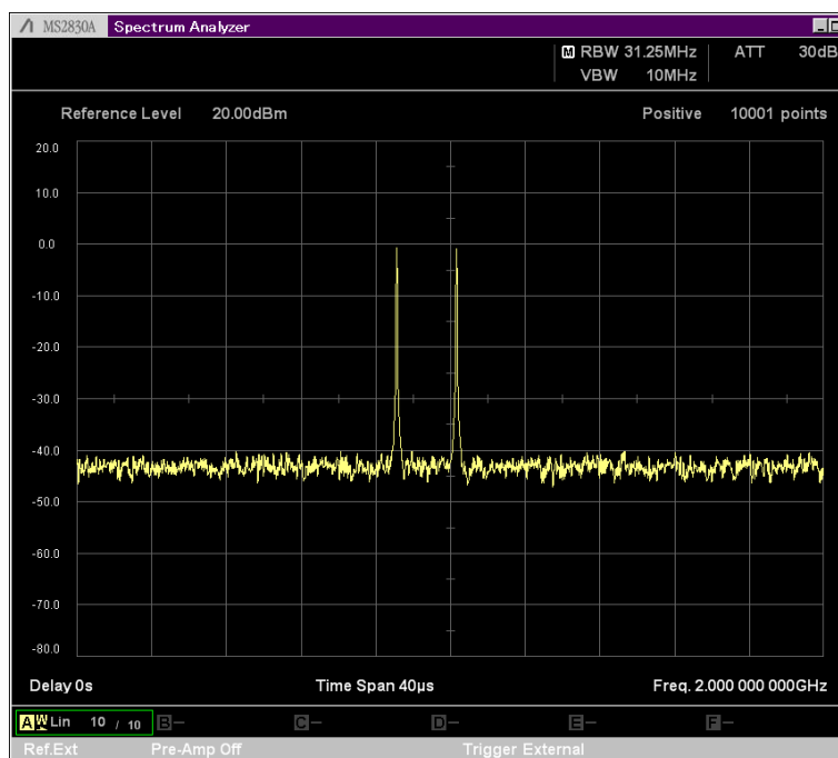
Figure 10. Status after second phase adjustment
