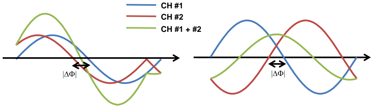
Figure 5. Waveforms of two signals to be synchronized; phase error \dots (left) and phase error 180^\circ + \dots (right)
