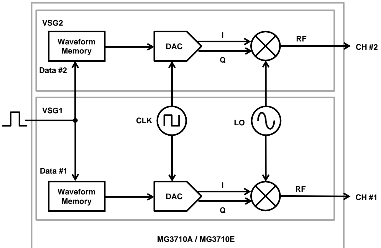
Figure 4. Channel synchronization using MG3710A / MG3710E
