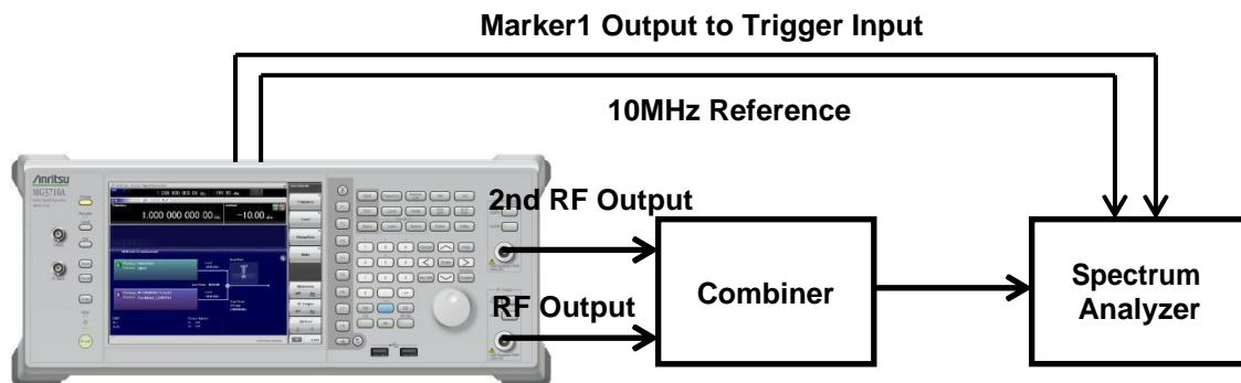
Figure 6. 2x2 MIMO configuration
