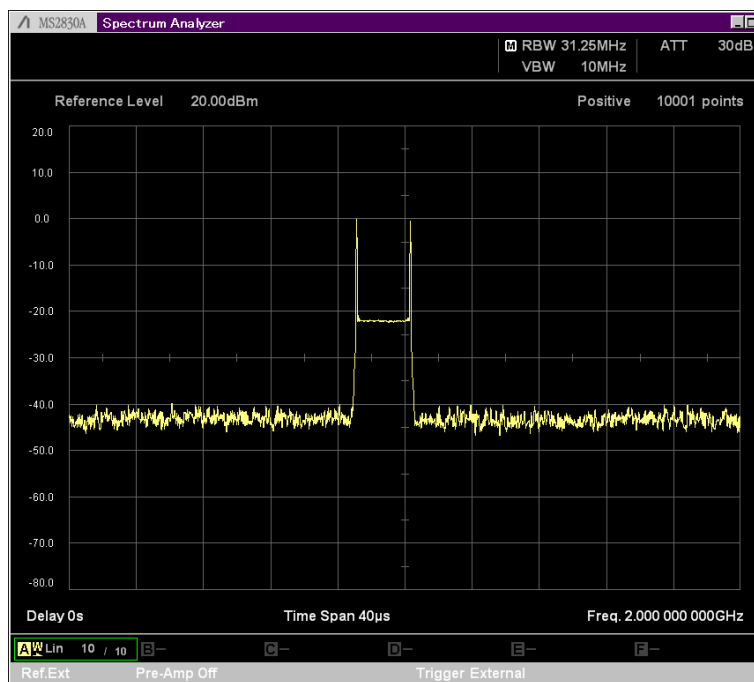
Figure 8. Status after first phase adjustment
