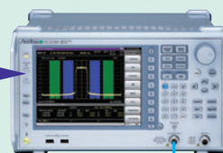
MS269xA Signal Analyzer + MS269xA-020 Vector Signal Generator (option)
