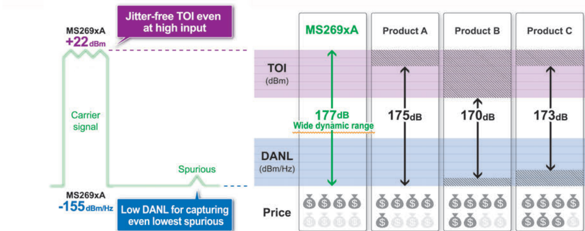
Distortion Characteristics (Spectrum Analyzer)
