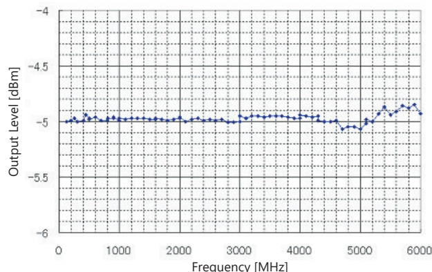
Example: Frequency Characteristics (Referenced to -5 dBm)
