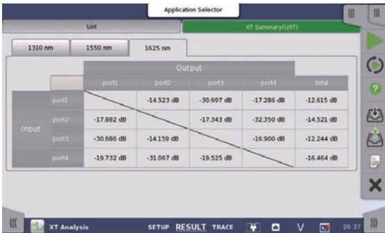
Far-end Crosstalk Between Cores
