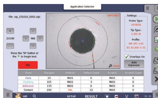
Optical connector End Face Test Judgment Window
