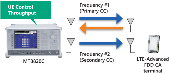
Example of MT8820C Connection
