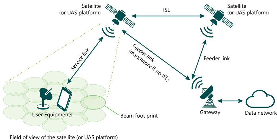
Regenerative Payload.
