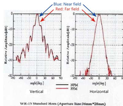
Near field/far field data comparison
