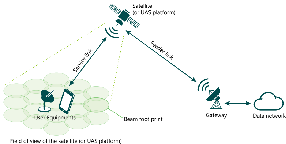
Transparent Payload.
