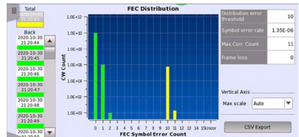
Bit Error Rate FEC Analysis
