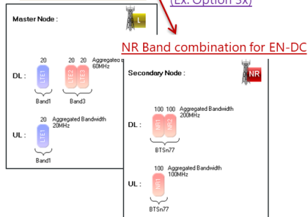
TDD Configuration Setup [Manual]
