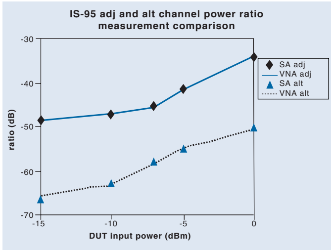
Figure 10. A comparison between measurements using a spectrum analyzer (SA) and using a Scorpion VNA (both using a PATS test set) is shown in this graph. The configurations were carefully setup to be comparable. The carrier frequency was 925 MHz.
