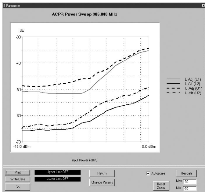
Figure 8. An example swept-power ACPR measurement is shown here for a narrowband CDMA (IS-95) input signal. Both upper and lower, adjacent and alternate channel measurements are shown.
