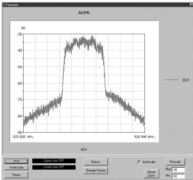
Figure 7. An example ACPR measurement of an amplifier at a single power is shown here using a narrowband CDMA (IS-95) input. The markers are positioned for channel measurements.
