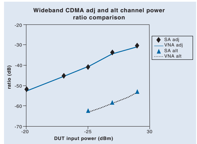
Figure 11. A comparison between measurements using a spectrum analyzer (SA) and using a Scorpion VNA (both using a PATS test set) is shown in this graph for a wideband CDMA configuration.
