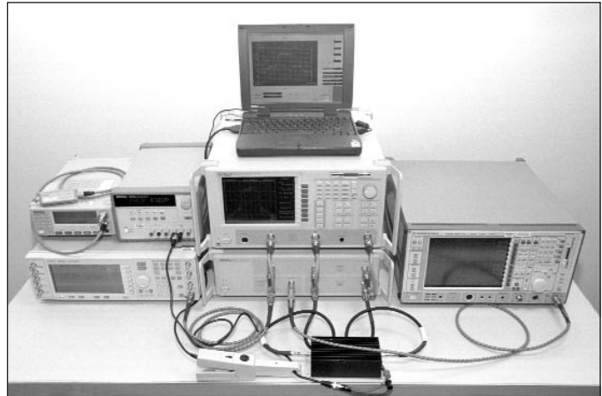
Figure 9. A typical correlation setup is shown here. An external modulated synthesizer and spectrum analyzer are simultaneously connected to facilitate correlation measurements.
