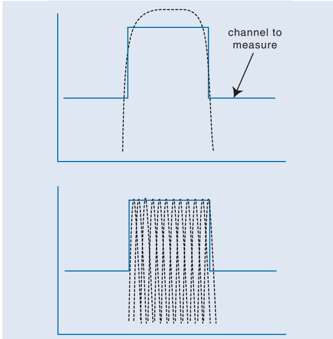
Figure 3. The difference between the single broadband measurement and multiple narrowband measurement approaches are schematically shown here. The wide measurement is faster but the effects of the measurement filter shape can be difficult to deconvolve. The measurement filter shape (shown as a dotted line) has less of an effect in the multiple measurement approach.
