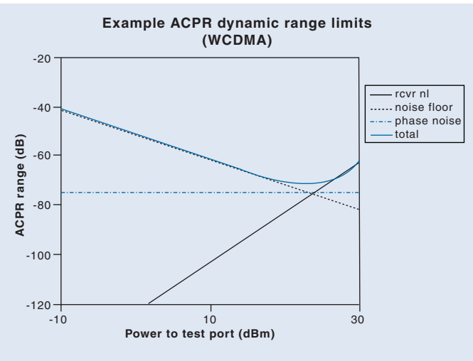
Figure 5. An example ACPR DR calculation for one type of wideband CDMA signal with the PATS/Scorpion configuration (0-dB receiver-side step attenuator setting) is shown here. Several assumptions go into this calculation but the optimal power range is between 0.1 and 1W for this setup. 'Power to test port' refers to power delivered into port 2 of the test set.
