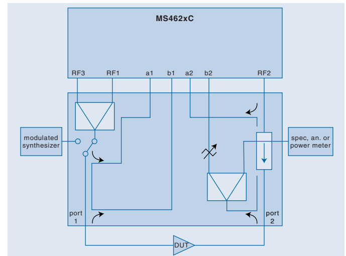
Figure 4. A standard PATS block diagram is shown here. An external modulated synthesizer is required for the ACPR measurement and models from several different manufacturers can be controlled by PATS software. An external spectrum analyzer and/or the Scorpion receiver can be used for making the ACPR measurements (both can be used for comparative measurements).
