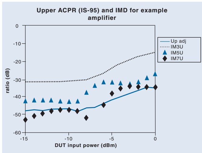
Figure 12. ACPR and IMD swept power measurements are shown here for an example amplifier. The products higher in frequency than the carrier are shown in this plot.
