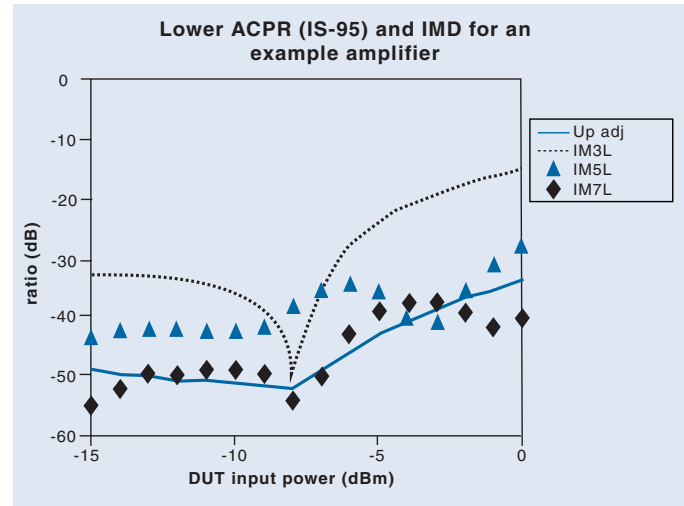
Figure 13. ACPR and IMD swept power measurements are shown here for an example amplifier. The products lower in frequency than the carrier are shown in this plot.
