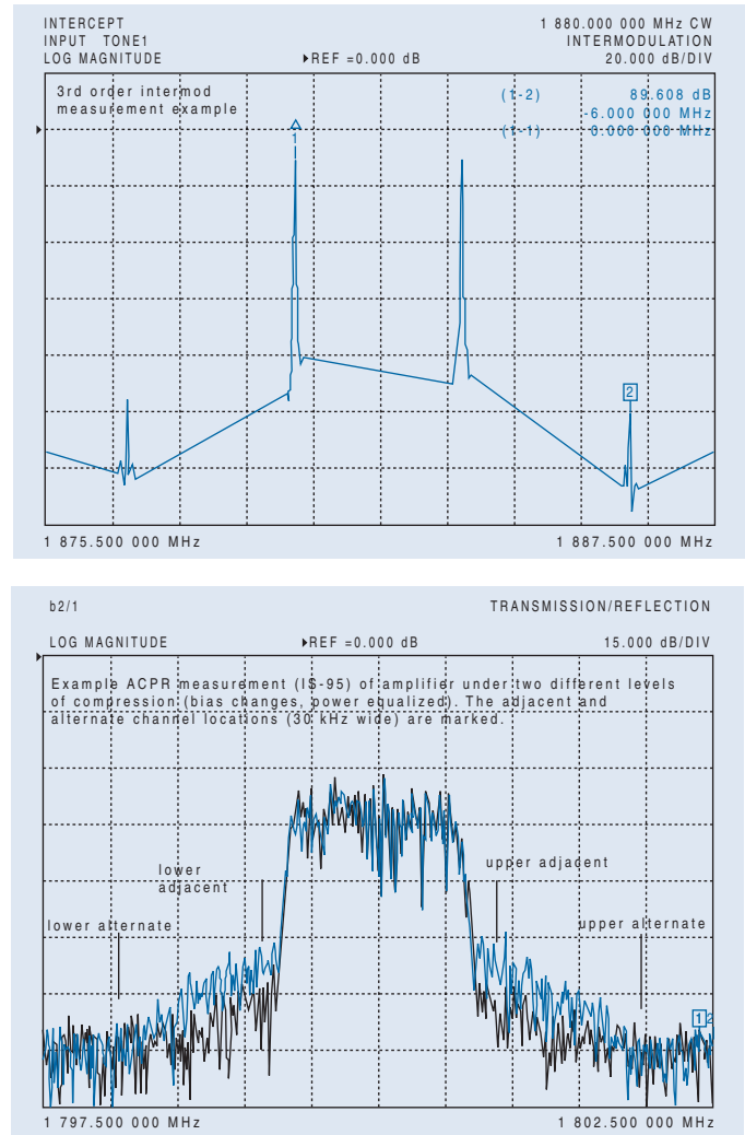
Figure 1. Example IMD and ACPR measurements are shown here. While the IMD measurement is simpler (requiring only 2 tones), it may do an inadequate job of predicting distortion performance under practical (i.e. modulated) conditions.
