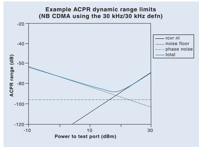
Figure 6. Another example dynamic range calculation with Scorpion/PATS and 0 dB attenuation is shown here, this time for a narrowband (IS-95) CDMA signal.
