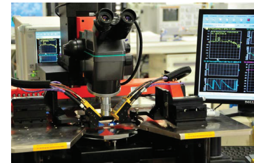
Improved measurement stability enables less frequent calibrations
