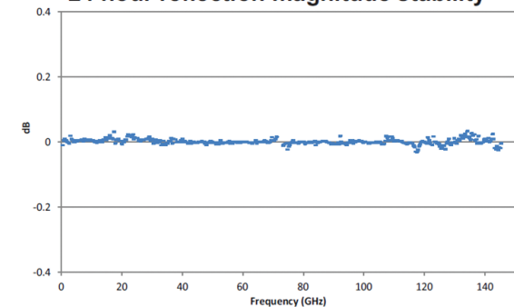
24 hour reflection magnitude stability
