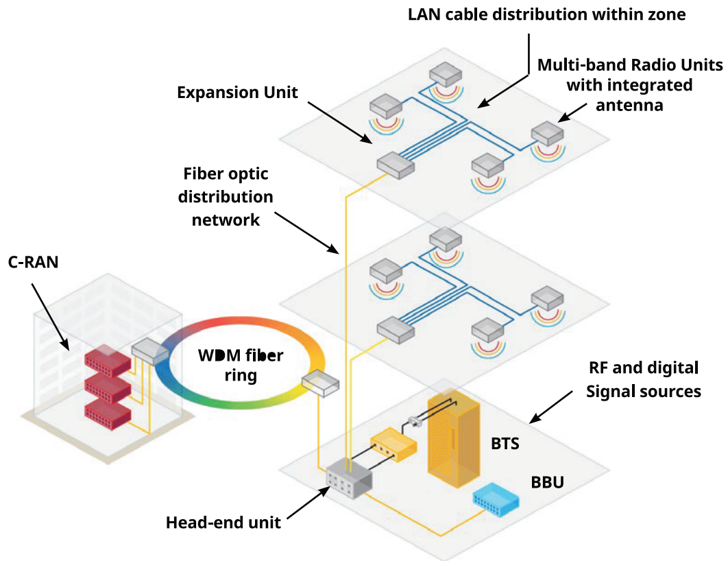
Figure 13. Digital DAS Configuration
