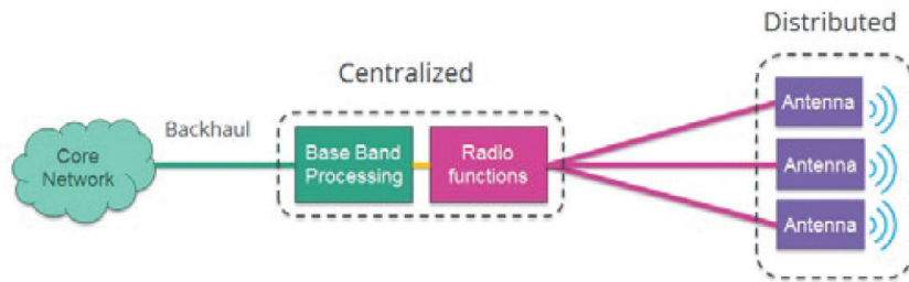
Figure 3. Distributed Antenna System (DAS) Architecture
