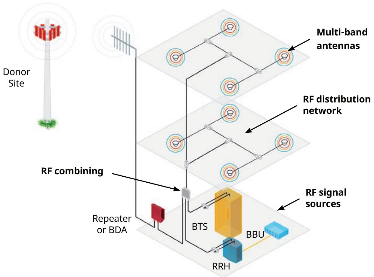
Figure 6. Passive DAS Configuration
