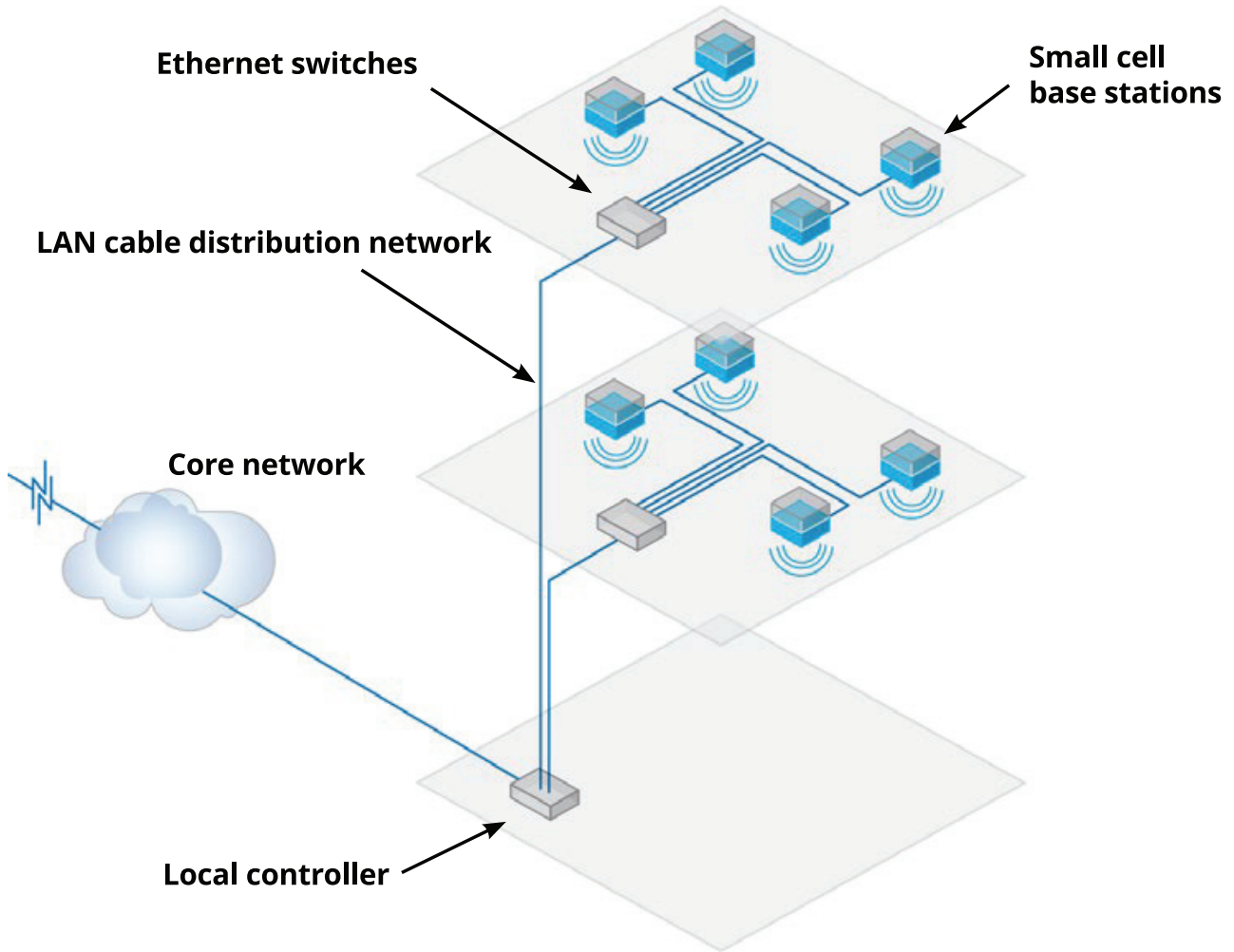
Figure 15. Distributed Small Cell (DSC) Configuration
