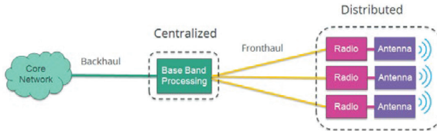
Figure 4. Distributed Radio System (DRS) Architecture
