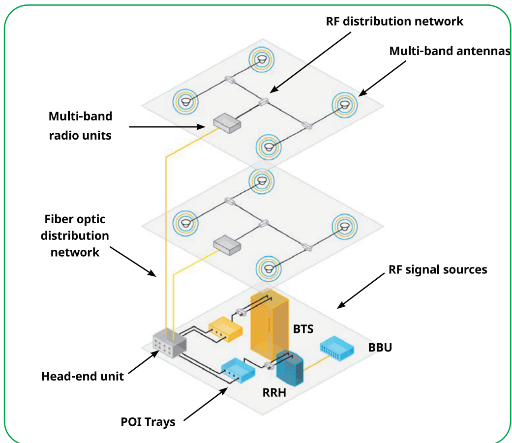
Figure 12. Hybrid DAS Configuration
