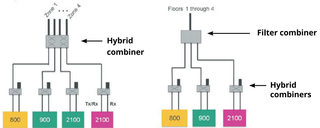
Figure 7. Passive DAS Combining Techniques
