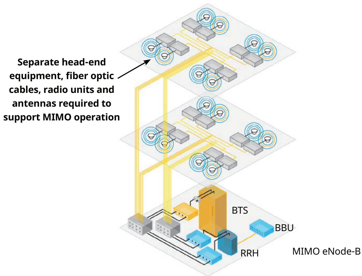
Figure 11. MIMO Active DAS Configuration
