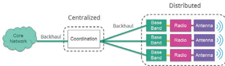
Figure 5. Distributed Small Cell (DSC) Architecture
