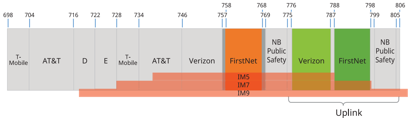
Figure 2. FirstNet Band 14
