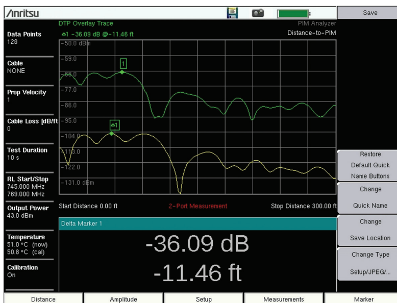
Figure 17. 2-Port DTP
