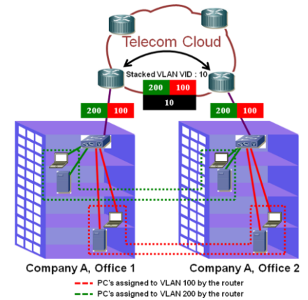
Figure 4. Example network of one company with two VLAN's.
