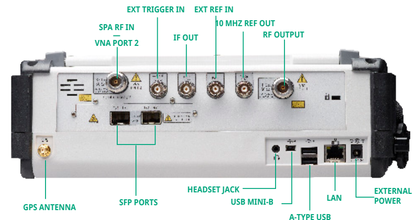
ALL CONNECTORS ARE CONVENIENTLY LOCATED ON THE TOP PANEL, LEAVING THE SIDES CLEAR FOR HANDHELD USE
