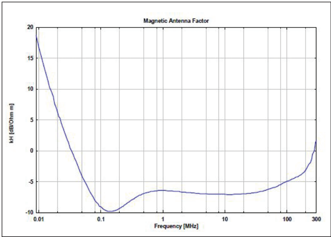
Magnetic Antenna Factor (typical)
