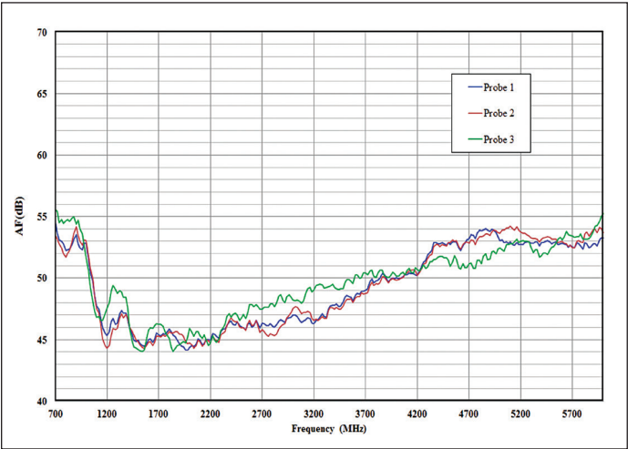
Antenna Factors (typical)
