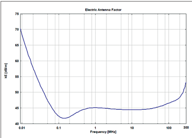
Antenna Factors (typical)
