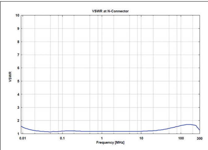
VSWR (typical)
