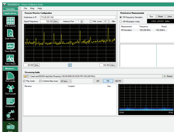
Figure 17. AM/FM Display for Measurements and Streaming
