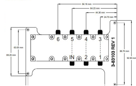
Picture of 6-port Multiplexer Module
