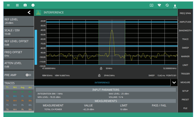
Interference Finder Option 24 Provides Fast Audio Tone Response to Changing Interference Levels
