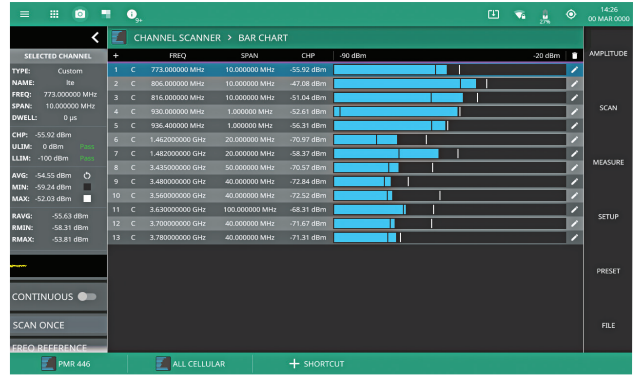
Bar Chart display monitoring GSM, LTE and 5G cellular bands
