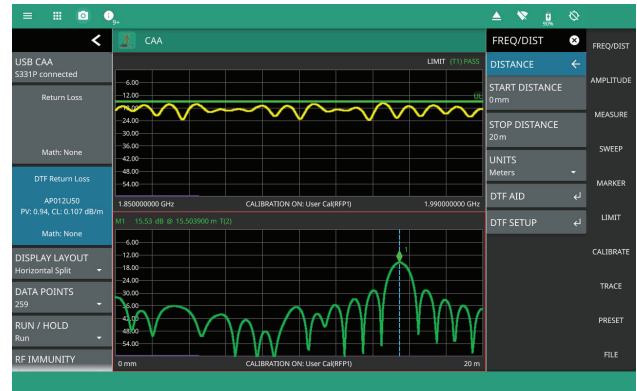
Simultaneous Display of Cable and Antenna Feed Return Loss and Distance to Fault
