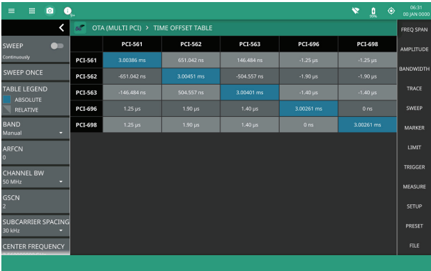
Time Offset Table Shows the Relative Time Offset between Signals Arriving From All gNB
