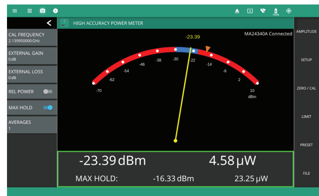
Option 19 Provides Power Meter Accuracy with a Large Analog Display Plus Digital Readout
