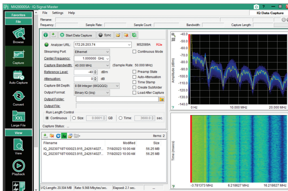
IQ Capture Screen Displays the Current Spectrum for which IQ Data will be Captured
