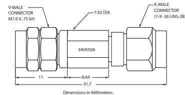
34VK50A outline
