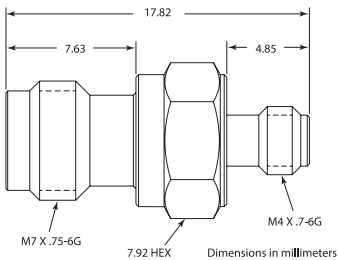
34WVVF50 outline
