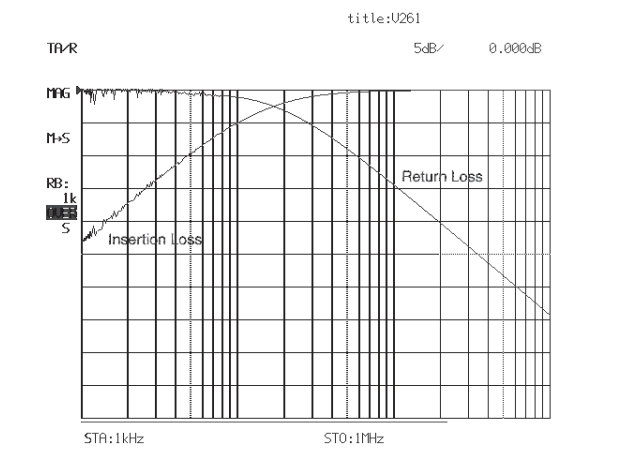
Typical Low Frequency Insertion Loss measured on V261 over the range of 1 kHz to 1 MHz.
