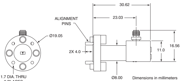
35WR10WF outline
