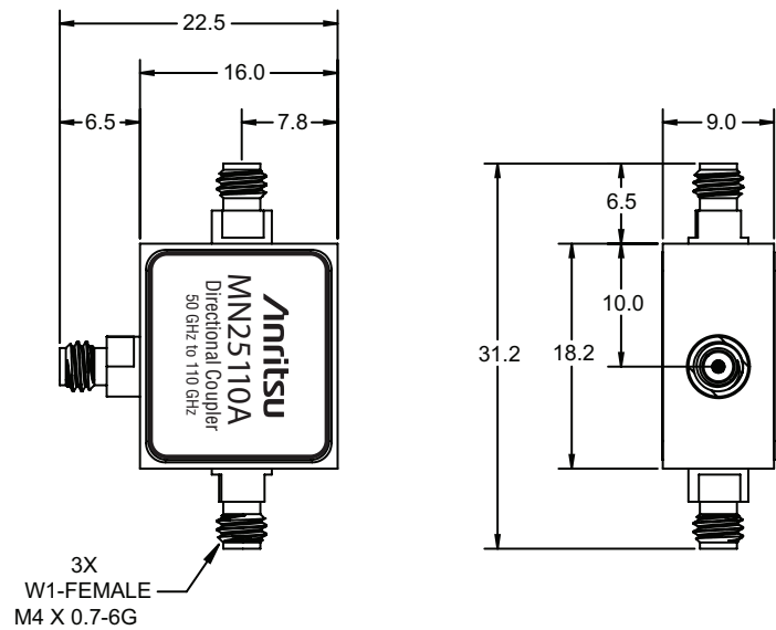
MN25110A outline
