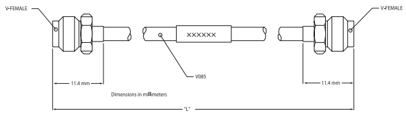
V120FF outline
