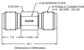
K222B outline
