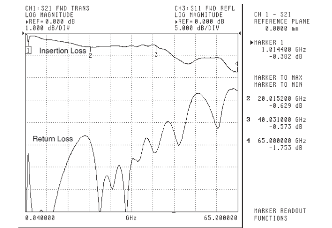
Insertion Loss and Return Loss measured on V261 over the range of 40 MHz to 65 GHz.
