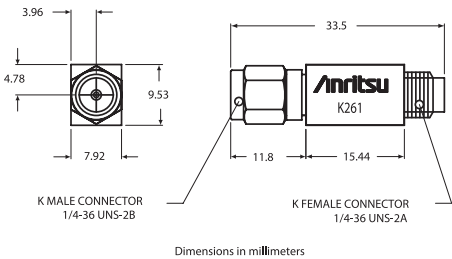
K261 outline
