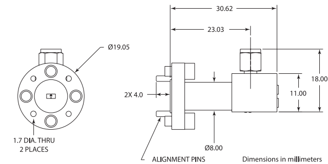
35WR10W outline
