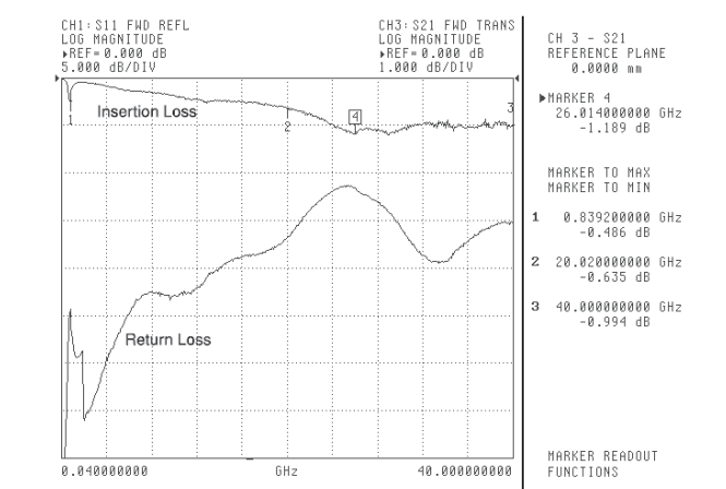
Insertion Loss and Return Loss measured on K261 over the range of 40 MHz to 40 GHz.
