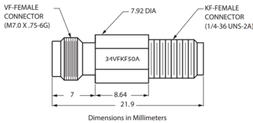
34VFKF50A outline
