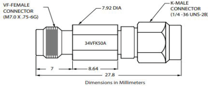
34VFK50A outline
