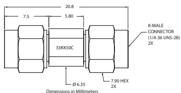
33KK50C outline
