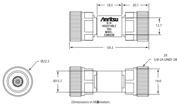
33NN50B outline
