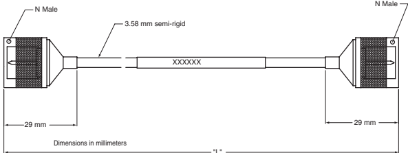
N120-6 outline
