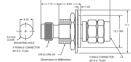
V234 outline
