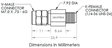
34VKF50A outline
