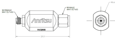
W265 outline
