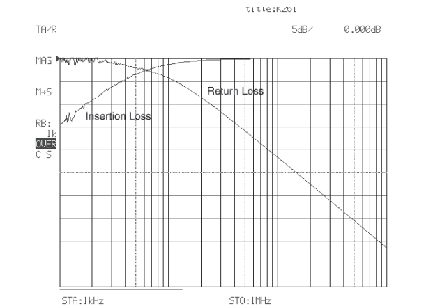
Typical Low Frequency Insertion Loss measured on K261 over the range of 1 kHz to 1 MHz.
