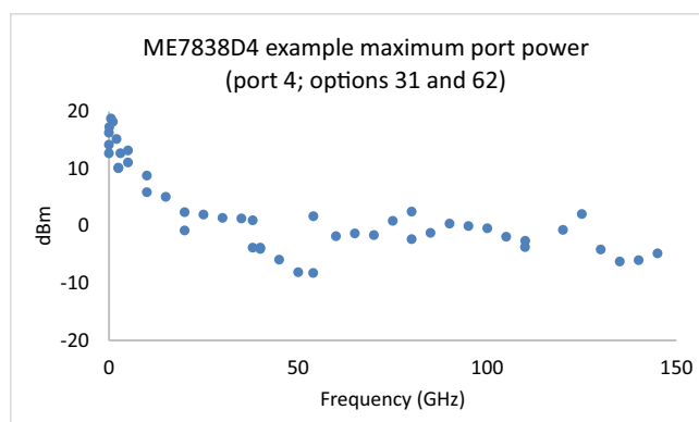
ME7838D4 4-Port Broadband Typical Maximum Port Power with options 31 and 62.
