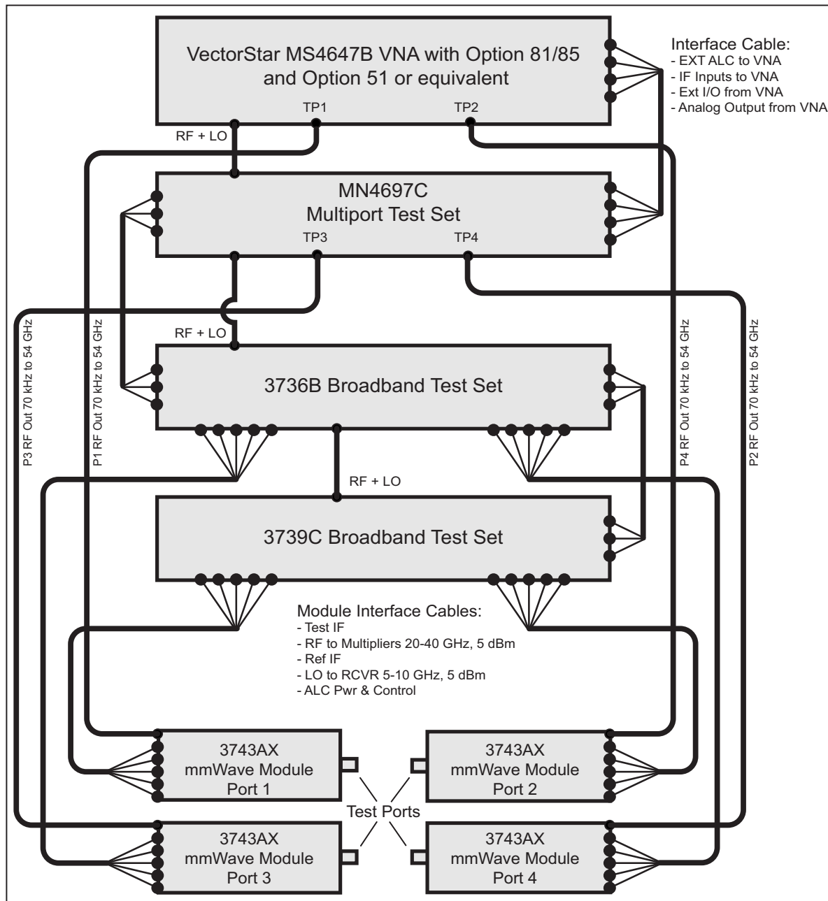
ME7838A4X Broadband 4-Port System
