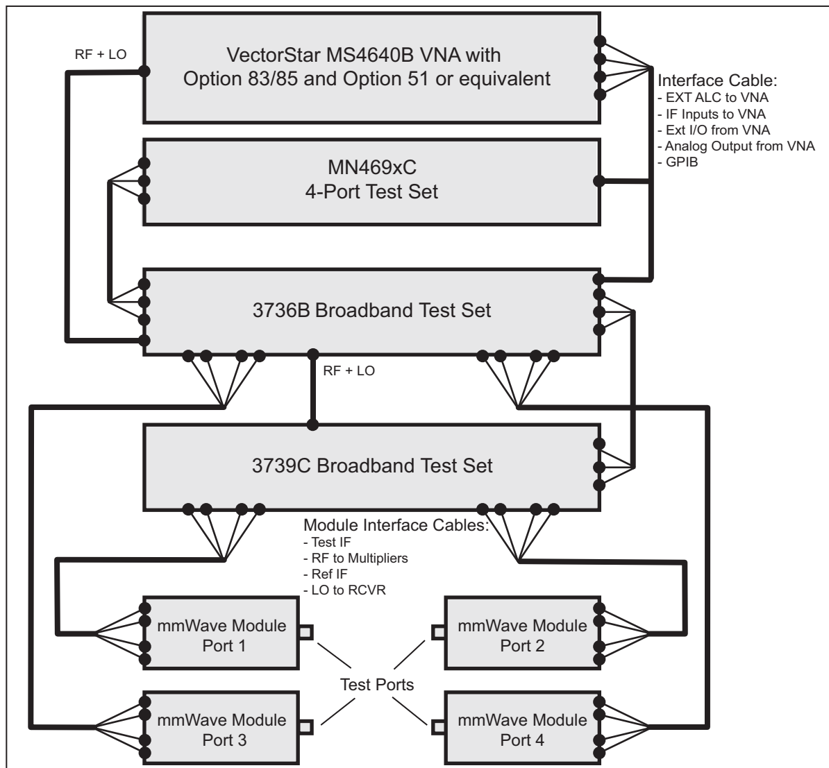
ME7838A4X Broadband 4-Port mmWave System
