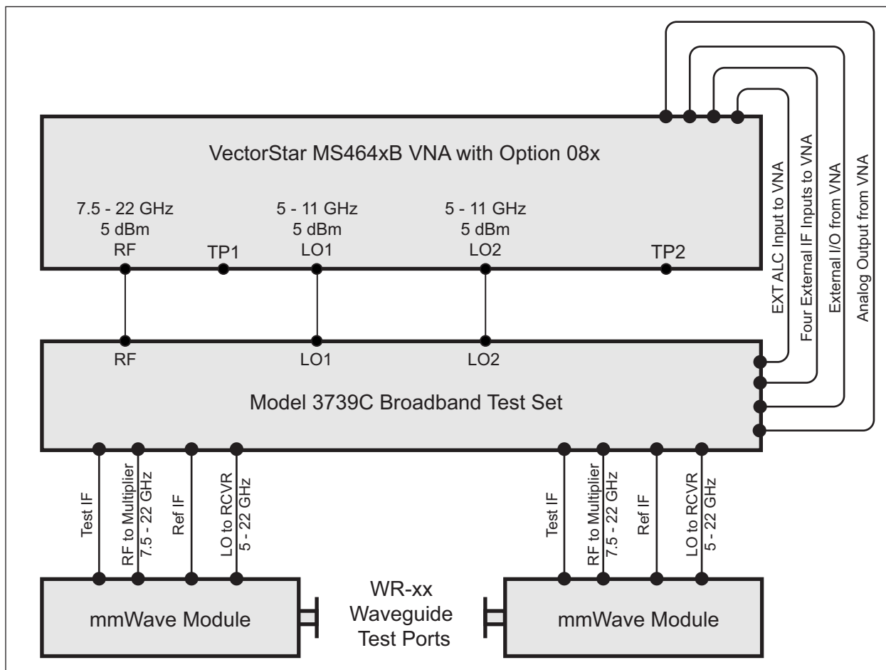
ME7838AX 2-port mmWave System
